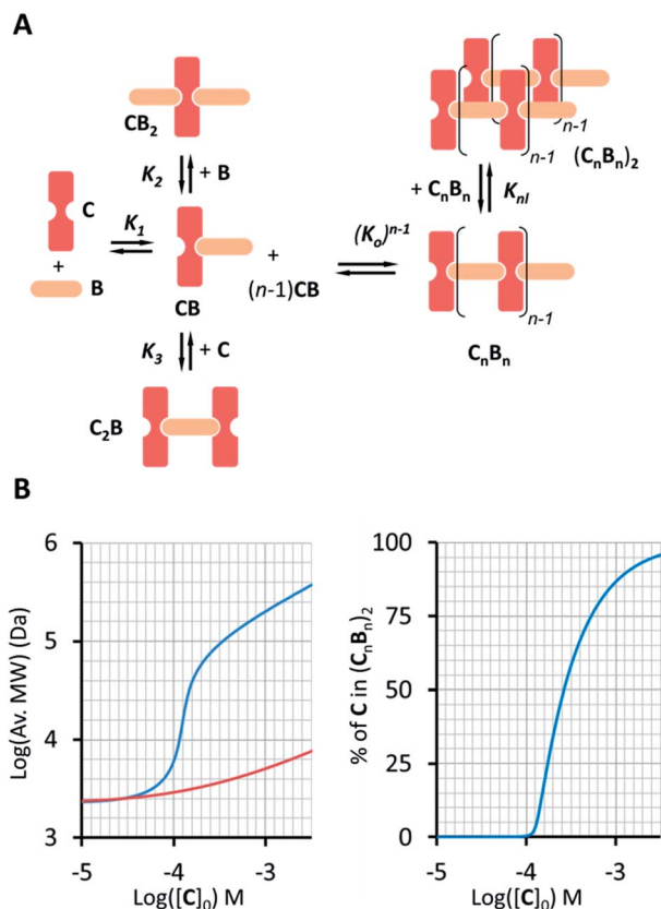
Fig. 4 (A) Equilibria that describe the oligomer dimerization model. (B) Left panel: changes in the average MW of the oligomer dimer ( (C_n B_n)_2 ) (blue trace) as the total concentration of C increases ( [B] = [C] ). For comparison, the increase in the average oligomer molecular weight in the absence of dimerization is also shown (red trace). The right panel shows the change in the percentage of C in (C_n B_n)_2 as a function of the total concentration of C.
