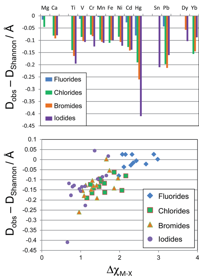
Fig. 2 Top, chart of deviation in experimental bond lengths from Shannon bond lengths in octahedral M–X bonds (X = halide) by element. Bottom, plot of deviation in experimental bond lengths from Shannon bond lengths against difference in electronegativity.
