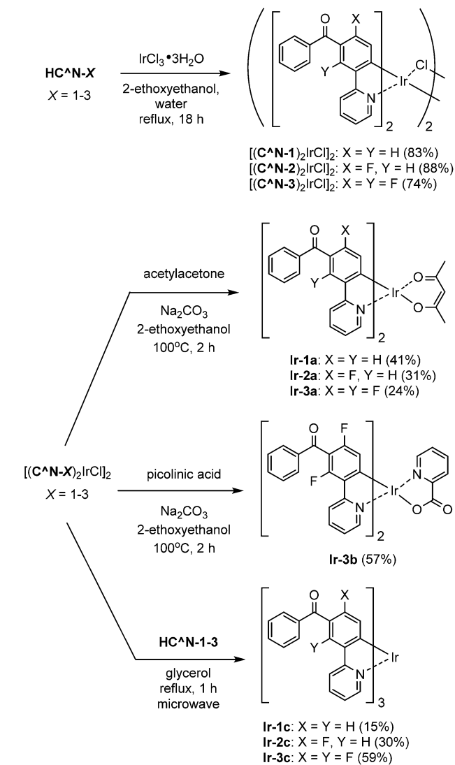
Scheme 2 Syntheses of iridium(III) complexes.
