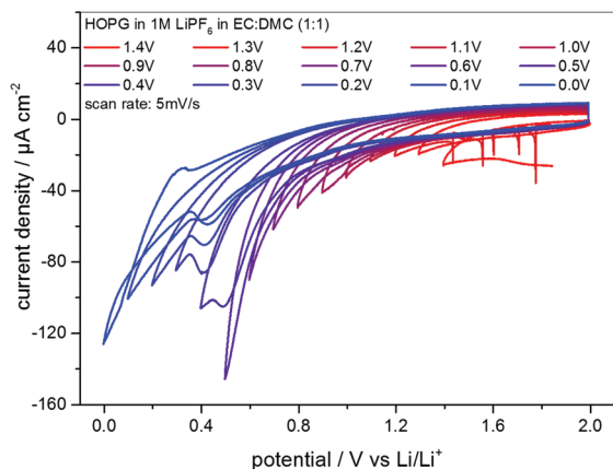
Fig. 5 Series of CVs of HOPG in 1 M \text{LiPF}_6 dissolved in EC/DMC (1:1). The lower vertex potential was decreased stepwise from 1.4 V to 0.0 V. Potential sweep rate: 5 \text{ mV s}^{-1} .
