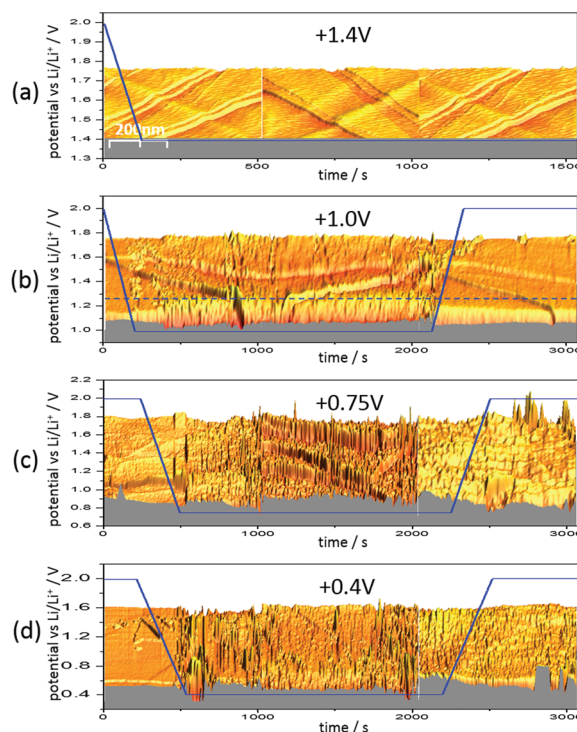
Fig. 6 In situ real time EC-STM images of HOPG in 1 M \text{LiPF}_6 in EC/DMC (1:1). The x-axis was converted to a time axis. Scan size: 500 nm by 500 nm; tunneling current: 500 pA; tip potential: 2.1 V; bias: variable; tip velocity: 1 \mu\text{m s}^{-1} for the experiment at 1.4 V and 0.5 \mu\text{m s}^{-1} for the other experiments; potential sweep rate: 5 \text{ mV s}^{-1} .
