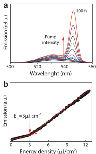
Fig. 4 Studies of lasing applications of \text{CH}_3\text{NH}_3\text{PbBr}_3 perovskite nano-wires: (a) amplified spontaneous emission (ASE) spectra of films prepared by a drop-casting technique from colloidal solution; (b) normalised ASE intensity versus energy density, and a linear fit intersection indicating a lasing threshold of 3 \pm 1 \mu\text{J cm}^{-2} .
