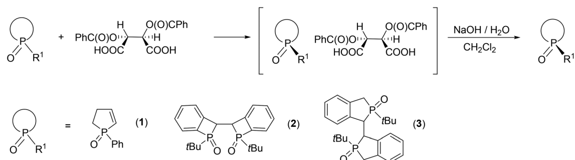
Fig. 2 Resolution of P-heterocyclic phosphine oxides using O,O'-dibenzoyl-(2R,3R)-tartaric acid.
