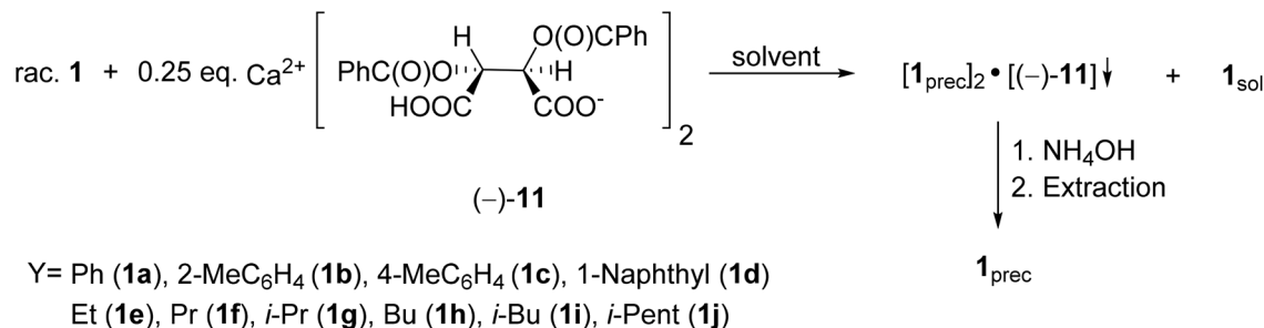
Scheme 12 General route for the resolution of 1-aryl- and 1-alkyl-3-methyl-3-phospholene 1-oxides ( 1a–j ) with \text{Ca}(\text{H-DBTA})_2 [(–)- 11 ].
