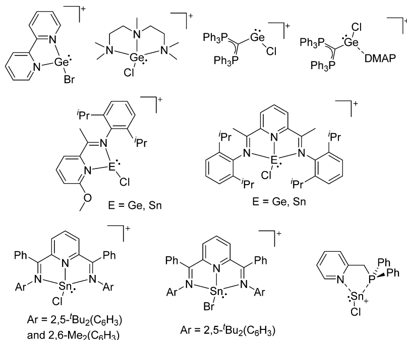
Fig. 55 Ligand-stabilized cations [(L)EX]^+ of germanium and tin.
