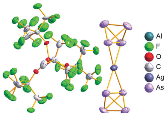
Fig. 65 Molecular structure of [\text{Ag}(\text{Asa})_2]_2^+[\text{Al}(\text{OR}^{\text{PF}})_4]^- . C. Schwarzmaier, M. Sierka, M. Scheer, Angew. Chem., Int. Ed. , 2013, 52 , 858–861. C. Schwarzmaier, M. Sierka and M. Scheer, Angew. Chem. , 2013, 125 , 891–894. Data from this reference were used to draw this figure. The disorder of the anion was omitted for clarity.
