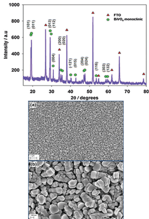
Fig. 35 XRD pattern of monoclinic BiVO 4 (green) on FTO (red) coated glass substrate deposited via AACVD; below: SEM image of BiVO 4 thin film at (a) 20 000 \times and (b) 100 000 \times . Reproduced with permission from ref. 248. Copyright 2012 Wiley.
