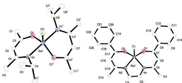
Fig. 21 ORTEP diagrams showing [Ga((Me)CN(H) t Pr)—CHC(Me)=O 2 Cl], left and [Ga((CH 2 ) 2 (N(H)C(Me)—CHC(C 6 H 5 )=O) 2 Me], right. Thermal ellipsoids are drawn at 50% probability. Reproduced from ref. 168 with permission from the Centre National de la Recherche Scientifique (CNRS) and the Royal Society of Chemistry.
