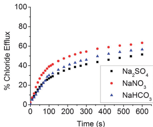
Fig. 3 Chloride efflux promoted by the addition of 5 (0.675 mol%) and either NaNO 3 or NaHCO 3 to the liposome solution (1 mM POPC, internal solution: 1 M NaCl, 0.1 M Na 2 SO 4 , 5 mM HEPES, pH = 7.2, external solution: 0.1 M Na 2 SO 4 , 5 mM HEPES pH = 7.2).
