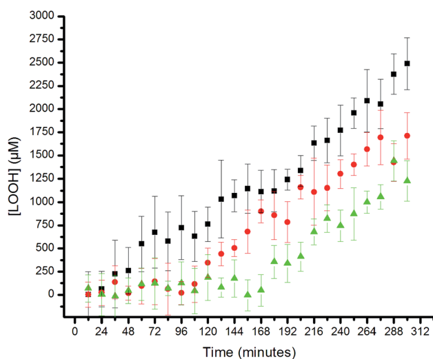
Fig. 5 Hydroperoxide formation in the autoxidation of 1-palmitoyl-2-linoleyl-sn-glycero-3-phosphocholine liposomes (13.3 mM in phosphate-buffered saline, pH 7.4) initiated by MeOAMVN (150 μM) at 37 °C in the presence of 25 μM 4 + 25 μM N-acetylcysteine (circles), 25 μM 4 + 50 μM N-acetylcysteine (triangles) or no additives (squares).
