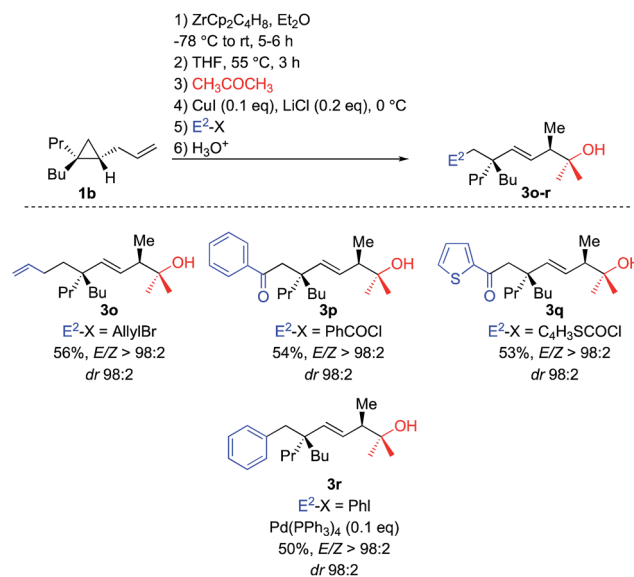
Scheme 5 Transmetalation of \text{Csp}^3\text{--}[\text{Zr}] bond for further C–C bond forming processes.
