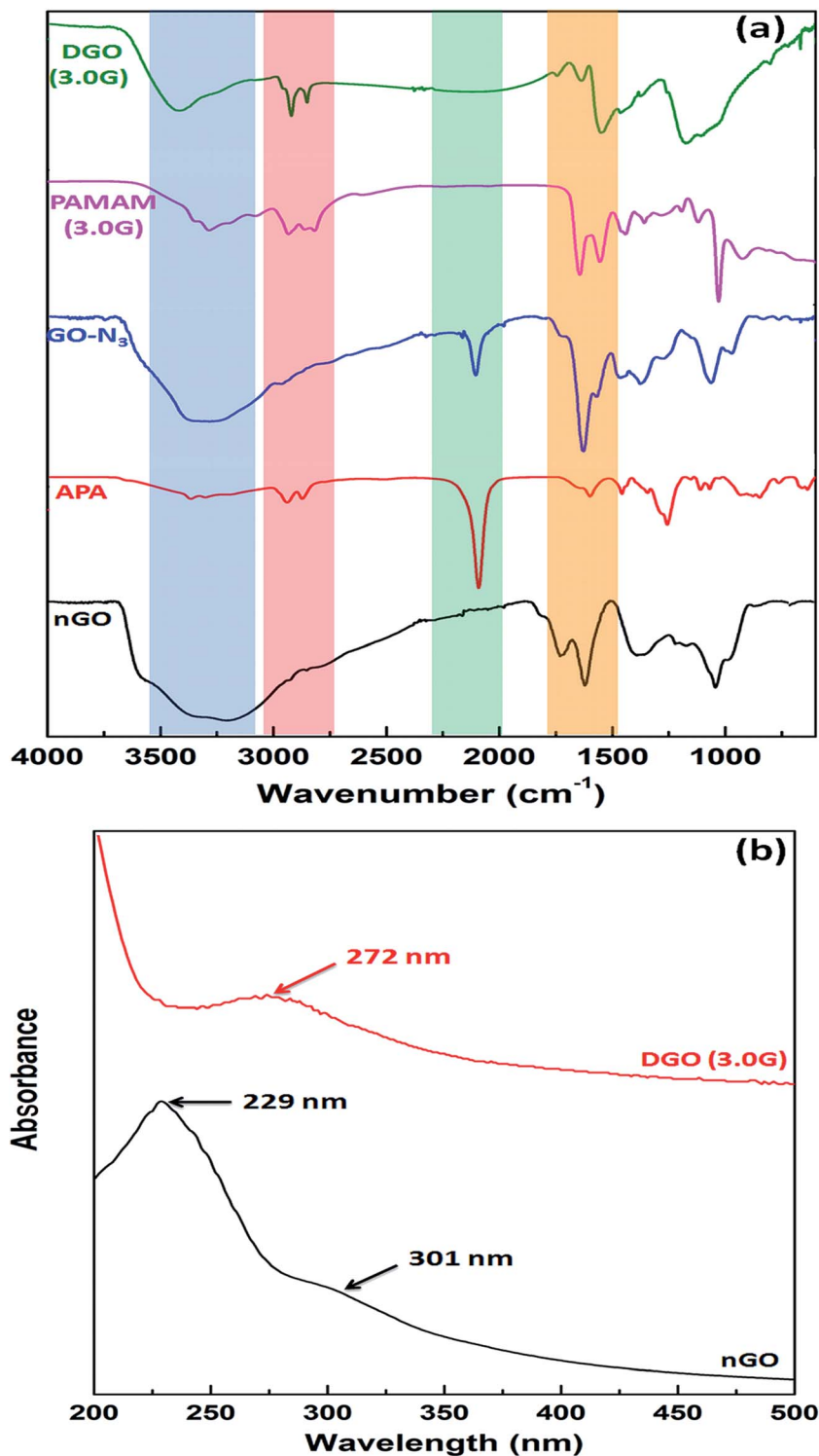
Fig. 2 (a) FTIR spectra of synthesized nGO, aminopropyl azide (APA), azide functionalized GO (GO-N 3 ), PAMAM dendrimer (3.0G) and dendronized GO (3.0G), and (b) UV-vis spectroscopy of nGO and DGO (3.0G).
