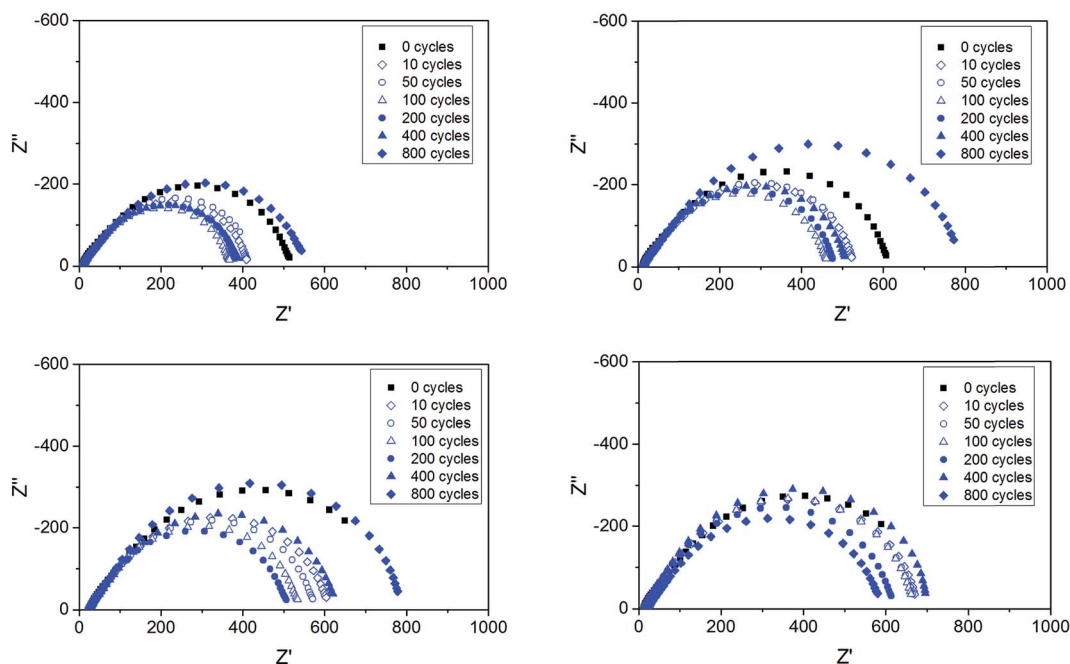
Fig. 10 Electrochemical impedance spectra of ternary electrolytes containing \text{Pyr}_{14}\text{TFSI} (left, top) and \text{Pyr}_{12\text{O}1}\text{TFSI} (right, top), \text{Pyr}_{14}\text{BETI} (left, bottom) and \text{Pyr}_{12\text{O}1}\text{BETI} (right, bottom) recorded at 21 ^{\circ}\text{C} during the plating–stripping cycle test at 40 ^{\circ}\text{C} . Frequency range: 100 kHz–1 Hz.
