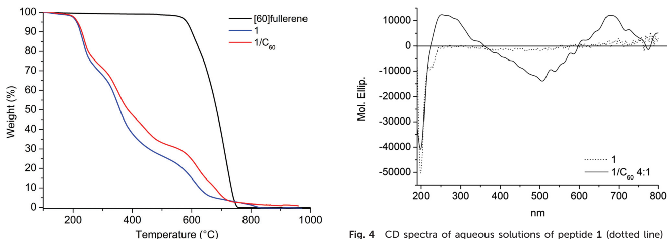
Fig. 3 TGA analysis (under a nitrogen atmosphere) of [60]fullerene, 1 and the 1/C 60 solution obtained by HSVM.
