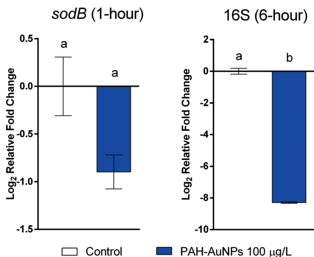
Fig. 4 In S. oneidensis , 16S gene expression decreased upon 100 µg L -1 PAH-AuNP exposure at long-term exposure (6 hour), while sodB gene expression did not show significant difference compared to control group. Error bars show standard error of the mean ( n \geq 4 ). Both figures follow the same legend. Different letter designations indicate significant difference between groups (unpaired t -test, \alpha = 0.05 ).
