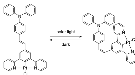
Scheme 2 Trans – cis isomerisation of complex \text{PtL}^2\text{Cl} .
