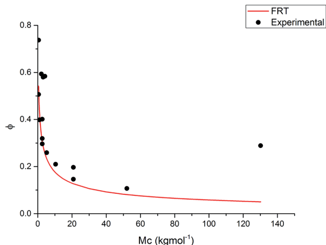
Fig. 9 The equilibrium volume fraction of polymer in the network of PS and DVB microgels in toluene at 25 °C over a range of molar masses between cross-links ( M_c ). Experimental data taken from ref. 20 and 36 (●). The line shows the theoretical predictions. \chi = 0.4 (ref. 62) and \bar{V}_1 = 105.91 \text{ cm}^3 \text{ mol}^{-1} .
