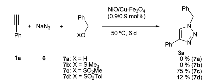
Scheme 1 Multicomponent cycloaddition with benzyl derivatives.
