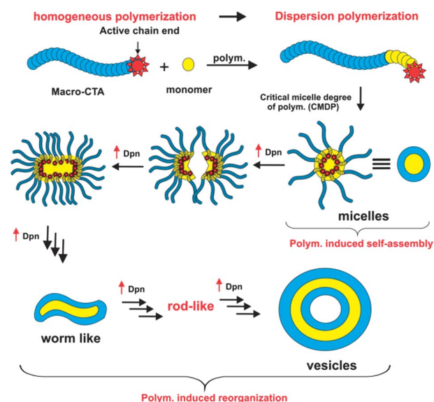
Scheme 2 Evolution of the self-assembly process as polymerization progresses.
