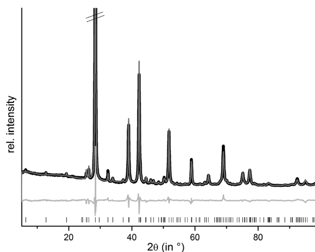
Fig. 2 Rietveld refinement of 21R\text{-Ge}_{0.5}\text{Sn}_{0.5}\text{Sb}_2\text{Te}_4 (the strongest reflection is cut off); vertical lines indicate calculated reflection positions, experimental (black) and calculated pattern (gray) and difference plot (below) are shown.
