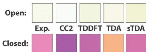
Fig. 3 Perceived colors of open and closed ring isomers as determined from the absorption spectra under daylight conditions. Colors are obtained from experiment and the different theoretical methods used.
