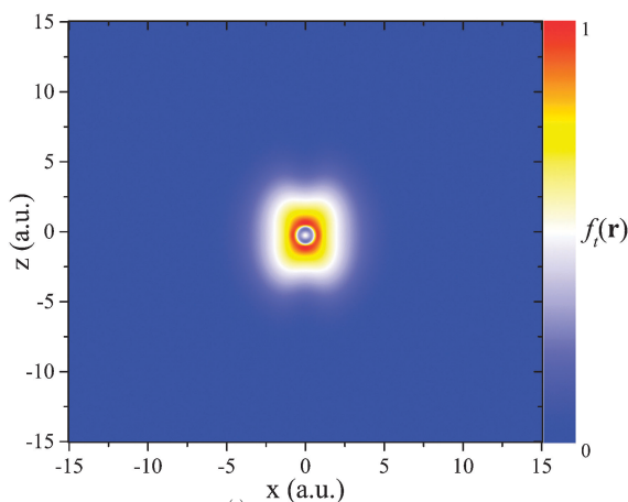
Fig. 5 The LMF f_i(\mathbf{r}) = \frac{1 - \frac{\tau_W(\mathbf{r})}{\tau(\mathbf{r})} \gamma^2(\mathbf{r})}{1 + c\gamma^2(\mathbf{r})} , evaluated with c = 0.5 , on the numerical grid for the C atom.
