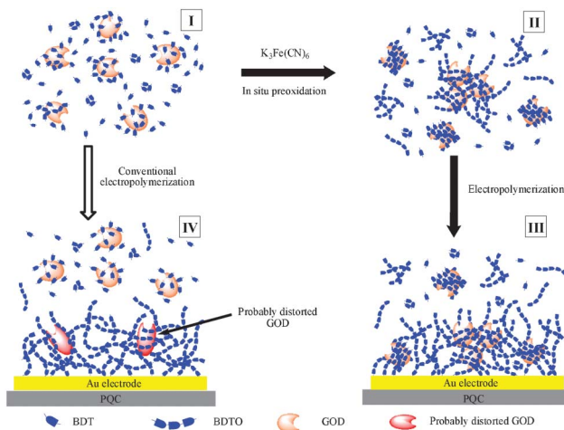
Fig. 3 Procedures for immobilization of GOx via the chemical preoxidation electropolymerization and conventional electropolymerization protocols. Reprinted with permission from ref. 160, copyright 2008, American Chemistry Society.
