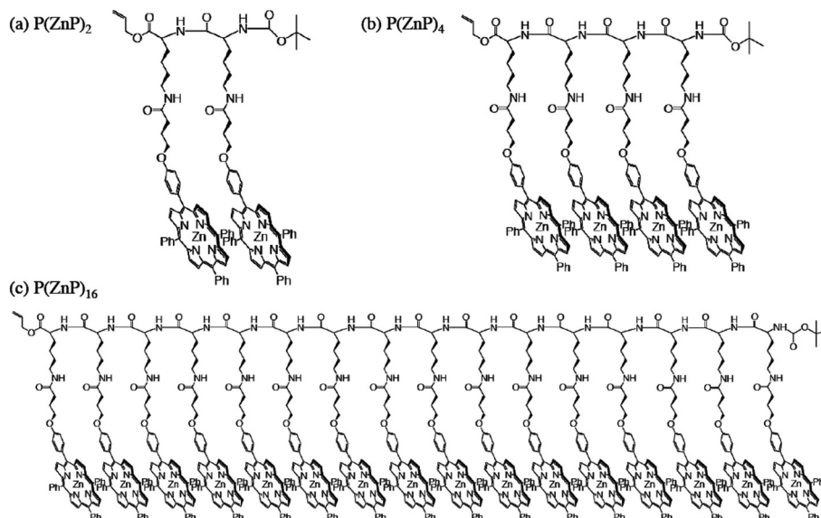
Fig. 14 Chemical structures of P(ZnP)_2 , P(ZnP)_4 and P(ZnP)_{16} .
