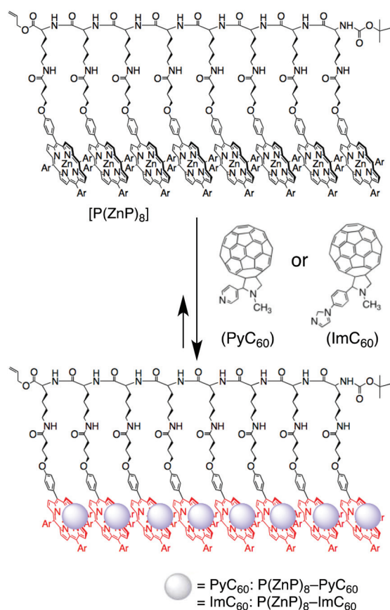
Fig. 15 Illustration of supramolecular complex composed of porphyrin-peptide octamer [P(ZnP) 8 , Ar = 3,5-( t -Bu) 2 C 6 H 3 ] and PyC 60 or ImC 60 .
