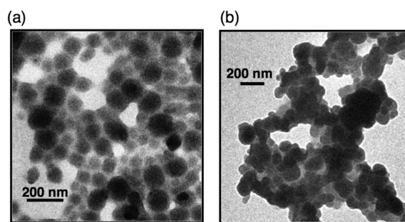
Fig. 4 TEM images of (a) \text{Li}^+@\text{C}_{60}/\text{ZnTPPS}^{4-} and (b) \text{Li}^+@\text{C}_{60}/\text{H}_2\text{TPPS}^{4-} nanoclusters.
