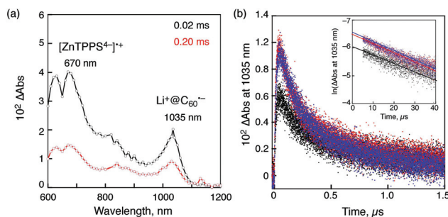
Fig. 2 (a) Transient absorption spectra of \text{ZnTPPS}^{4-} ( 2.5 \times 10^{-5} M) in the presence of \text{Li}^+@C_{60} ( 5.0 \times 10^{-5} M) in deaerated PhCN at 298 K taken at 20 and 200 \mu\text{s} after nanosecond laser excitation at 550 nm; (b) decay time profiles at 1035 nm with different laser intensities (1, 3, 6 mJ per pulse). Inset: first-order plots.
