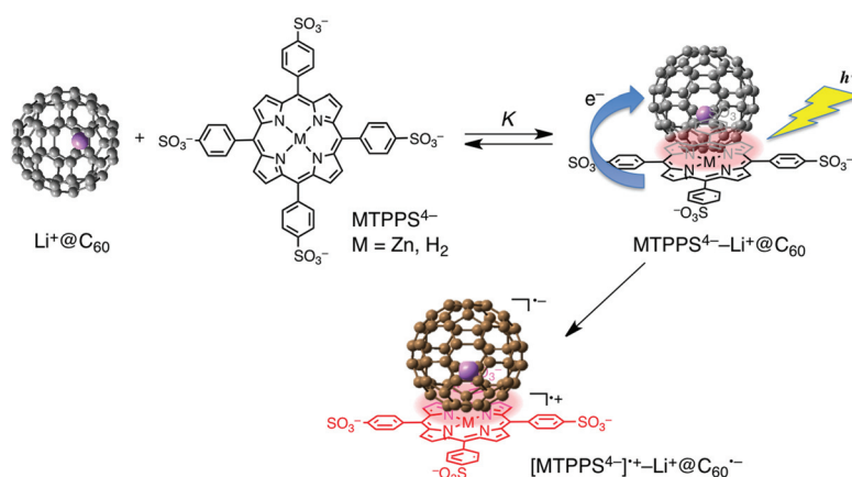
Scheme 1 Supramolecular complex formation and photoinduced charge separation of MTPPS 4− (M = Zn and H 2 ) with Li + @C 60 in PhCN.
