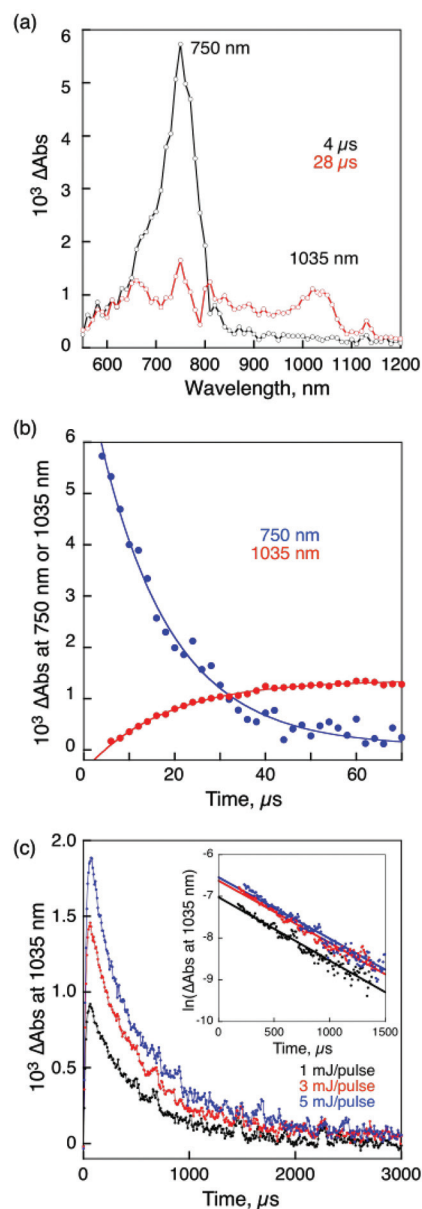
Fig. 10 (a) Transient absorption spectra of \text{Ni}_2\text{-CPDpy}(\text{OC}_6) with \text{Li}^+@C_{60} in deaerated PhCN at room temperature taken at 4 and 28 \mu\text{s} after nanosecond laser excitation at 520 nm. [\text{Ni}_2\text{-CPDpy}(\text{OC}_6)] = 2.5 \times 10^{-5} M, [\text{Li}^+@C_{60}] = 5.0 \times 10^{-5} M. (b) Rise and (c) decay time profiles at 1035 nm with different laser intensities (1, 3, 5 mJ per pulse). Inset: first-order plots.
