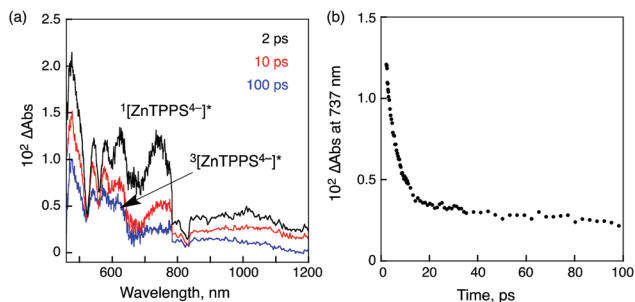
Fig. 1 (a) Transient absorption spectra of \text{ZnTPPS}^{4-} ( 2.5 \times 10^{-5} \text{ M} ) in the presence of \text{Li}^+ @ \text{C}_{60} ( 5.0 \times 10^{-5} \text{ M} ) in deaerated PhCN at 298 K taken at 2, 10 and 100 ps after femtosecond laser excitation at 388 nm. (b) Time profile at 737 nm.
