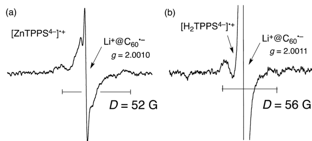
Fig. 3 EPR spectra of (a) (\text{ZnTPPS}^{4-})^{*-}\text{Li}^{+}@\text{C}_{60}^{*-} and (b) (\text{H}_2\text{TPPS}^{4-})^{*-}\text{Li}^{+}@\text{C}_{60}^{*-} in PhCN generated by photoirradiation with a high-pressure Hg lamp (1000 W) at 77 K.
