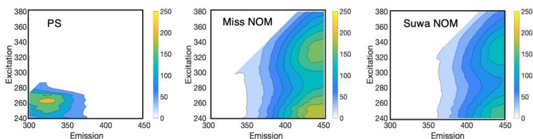
Figure 7. EEM comparison of PS and DOM from Suwannee and Mississippi Rivers. All samples have a DOC concentration of 32 mg L -1 . Intensity values are triplicates for each NOM samples and PS.
