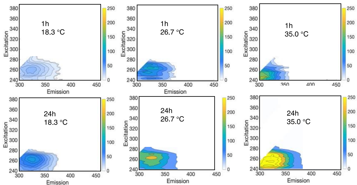
Figure 5. EEM comparison of PS at 35.0, 26.7 and 18.3 °C after 1 h (top) and 24 h (bottom) irradiation. It should be noted that different temperature graphs have different intensity ranges to pronounce the changes in EEM. Intensity is arithmetic mean of triplicates for each temperature and at each time interval.
