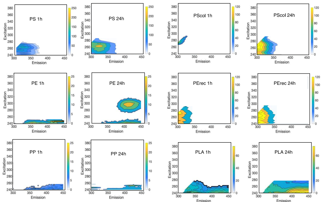
Figure 3. Fluorescence analysis using excitation (240-400 nm) and emission (300-450 nm) after 1 h UV irradiation and 24 h UV irradiation. 24 h intensity values are arithmetic mean of triplicate experiments for PS and PE and arithmetic means of triplicate measurements of other polymers.
