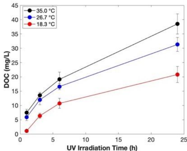
Figure 4. DOC formation kinetics comparison of PS at 35.0, 26.7 and 18.3 °C after 24 h irradiation. Error bars represent one standard deviation of triplicate experiments for each temperature.
