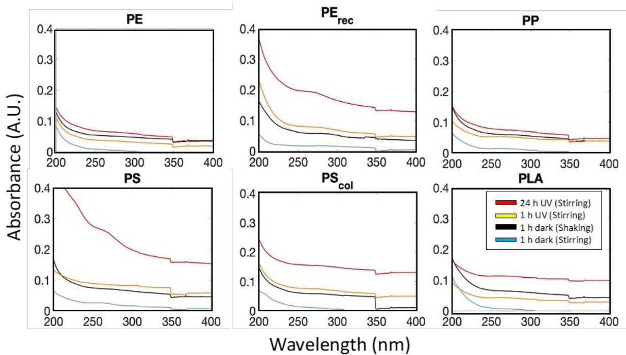
Figure 1. UV absorbance of leachate solutions for six types of microplastics aged by 24 h and 1 h UV irradiation and associated 1 h dark controls (i.e., stirring, and turbulent shaking). Absorbance values of 1 h and 24 h UV aging are arithmetic mean of triplicate experiments for PS and PE and arithmetic means of triplicate measurements of other polymers. Dark conditions and stirring control are mean of triplicate experiments for all polymers.
