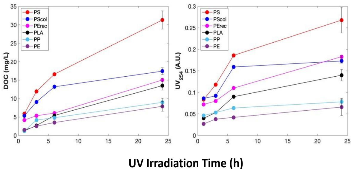
Figure 2. UV 254 absorbance (right) and DOC concentration in mg L -1 (left), for UV irradiated samples taken at 1, 3, 6, and 24 h. Error bars represent standard deviation of triplicate experiments for PE and PS, and triplicate measurements for the other polymer types. A comparison figure of UV 254 and DOC results for each polymer after 24 h is presented in the supplementary information (Figure S5). Lines are drawn to guide the eye.
