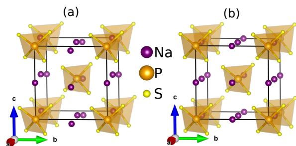
Fig. 1 The crystal structure of (a) low temperature tetragonal phase (P-421c) and (b) high temperature superionic cubic (I4-3m) phase of \text{Na}_3\text{PS}_4 .
