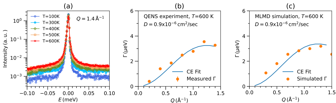
Fig. 4 (a) Temperature dependent QENS spectra of Na 3 PS 4 , measured at Q = 1.4 \text{ \AA}^{-1} (integrated over \delta Q = 0.2 \text{ \AA}^{-1} ). (b) The measured Q -dependence of \Gamma (orange markers) fitted with Chudley-Elliott jump-diffusion model (solid line). (c) The calculated \Gamma obtained by fitting the Lorentzian to simulated S_{\text{inc}}^{\text{Na}}(Q, E) (dots) using NVT-MLMD trajectories with 0.6% Na-vacancy in Na 3 PS 4 and Chudley-Elliott fit (solid line).
