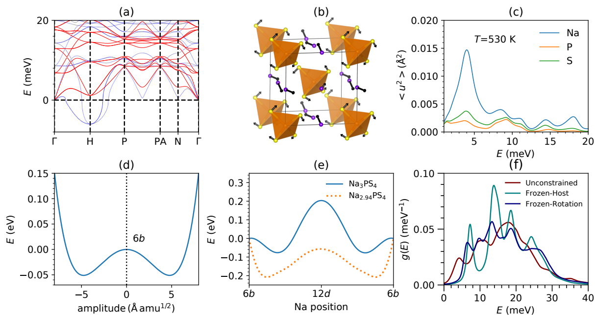
Fig. 3 (a) Calculated phonon dispersions at T=0 K under QHA (dotted blue lines) and at 600 K using anharmonically renormalized force-constants (solid red lines) in the cubic phase of \text{Na}_3\text{PS}_4 . (b) The eigenvector of the lowest unstable phonon mode at H -point ( 1/2 1/2 1/2 ) in cubic- \text{Na}_3\text{PS}_4 . (c) Calculated \langle u^2 \rangle as a function of phonon energy E averaged over entire Brillouin zone at 530 K in the cubic phase of \text{Na}_3\text{PS}_4 . The modes below 10 meV significantly contributed to Na vibrations and \text{PS}_4 librations. (d) The calculated energy profile of the lowest unstable phonon mode at H -point ( 1/2 1/2 1/2 ) in cubic- \text{Na}_3\text{PS}_4 . The vertical dashed line represent the configuration where all the Na atoms are at 6b sites (e) NEB calculation of energy barrier profile for Na migration between 6b crystallographic sites in stoichiometric phase (solid blue line) and 2% Na-vacant (dotted orange lines). The lowest phonon energy profile near 6b shown in (d) closely follows the stoichiometric NEB profile near 6b . (f) The calculated Na phonon DOS from NVT-MLMD in unconstrained, frozen-host (with only Na atomic degree of freedom) and frozen-rotation ( \text{PS}_4 rotational degree are frozen, while \text{PS}_4 translations are allowed) simulation environment at 600 K. Constraining \text{PS}_4 dynamics results in suppression of low- E modes around \sim 3 -5 meV.
