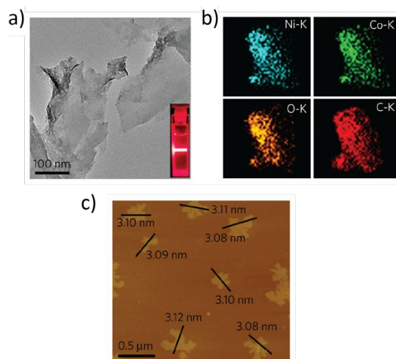
Fig 7. a) TEM image of NiCo-UMOFNs with optical image of Tyndall light scattering (inset) upon laser irradiation. b) EDS elemental mapping of NiCo-UMOFNs obtained within a TEM. c) AFM map of individual NiCo-UMOFN flakes. Adapted by permission from Springer Nature. 115 Copyright 2016.
