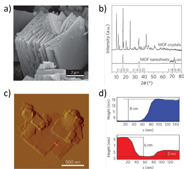
Fig 8. a) SEM image of bulk CuBDC MOF crystals comprised of layered nanosheets. b) pXRD scans of bulk CuBDC MOF crystals and corresponding nanosheets. c) AFM map of MOF nanosheets. d) Height profiles taken along the paths indicated in c. Adapted by permission from Springer Nature. 75 Copyright 2015.
