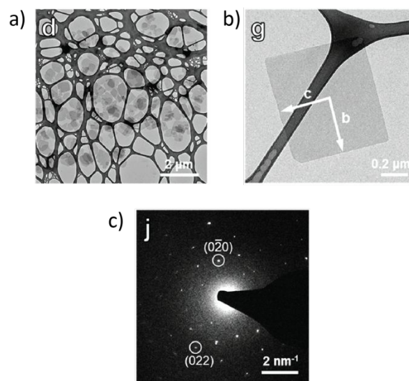
Fig 3. TEM images of a) several nanocrystals and b) a single nanocrystal of Zn(Bim)OAc synthesized in a suspension of CTAB in heptane and hexanol at 25 °C. c) Corresponding electron diffraction pattern of a single nanocrystal. Adapted with permission. 78 Copyright 2018 American Chemical Society.
