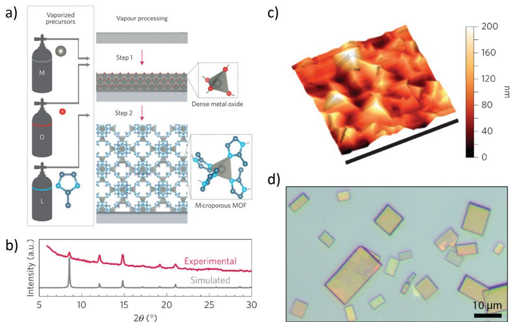
Fig 6. a) Schematic representation of CVD synthesis of ZIF-8 through a two-step process involving deposition of a dense metal oxide followed by introduction of organic ligand. b) Conversion of ZnO to ZIF-8 confirmed via comparison of measured and simulated pXRD patterns. c) 3D rendered AFM topograph of a polycrystalline film of ZIF-8. d) Optical images of single crystals of our \text{Mo}_2(\text{INA})_4 MOF synthesized directly through a one-step CVD reaction. 112 Adapted by permission from Springer Nature 110 Copyright 2016.
