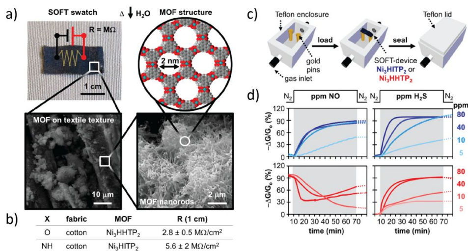
Fig 11. a) Conductive SOFT-devices produced from solvothermal condensation of MOF reagents in water onto textiles. Photograph of SOFT-device (top left), SEM images of textile fibers coated by MOF film (bottom left), SEM image of characteristic MOF nanorod structure (bottom right), and space-filling model of MOF (top right). b) Sheet resistance measurements for SOFT-devices. c) Schematic of custom enclosure for measuring d) response of SOFT-sensors when exposed to NO (left) or H 2 S (right). Adapted with permission. 181 Copyright 2017 American Chemical Society.
