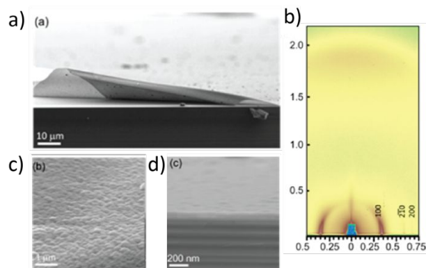
Fig 5. a) Highly uniform thin film of LZU-1 synthesized with in situ deprotection. b) The crystallinity and orientation are confirmed by GIWAXS. c) The thin film is composed of small crystallites with similar orientation and is 190 nm thick as measured by d) cross-sectional SEM. Adapted with permission. 101 Copyright 2017 American Chemical Society.
