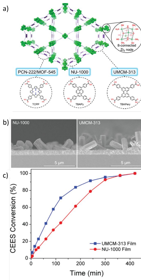
Fig 13. a) General structure of three MOFs, PCN-222/MOF-545, NU-1000, and UMCM-313, used as a thin-film protective coating against mustard gas simulant. b) NU-1000 and UMCM-313 thin films prepared using layer-by-layer techniques on FTO substrates and c) their reaction profiles for the photocatalytic oxidation of CEES. Adapted with permission. 226 Copyright 2018 American Chemical Society.
