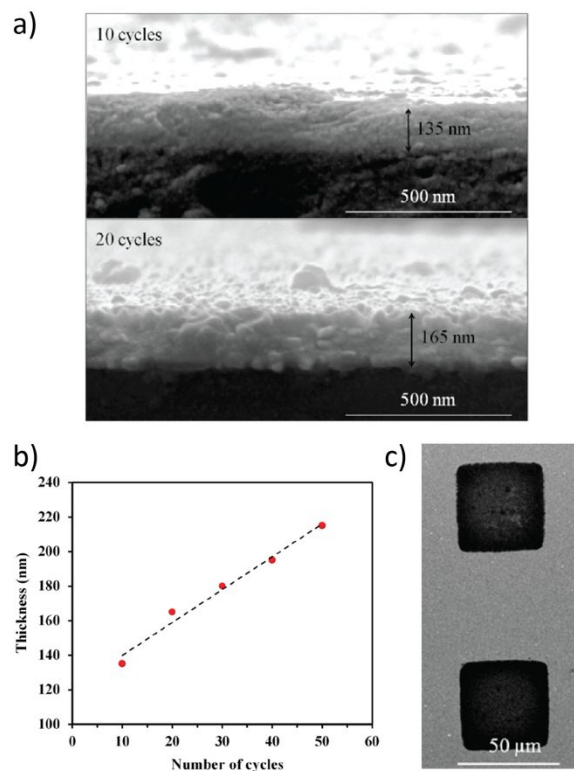
Fig 4. a) SEM images of the cross-section of \text{Cu}_2(\text{bdc})_2 \cdot x\text{H}_2\text{O} MOF thin films deposited using the four micro-syringe spin-coating method after 10 (top) and 20 (bottom) cycles. b) Height profiles of thin films produced after 10 to 50 cycles. c) Substrate-selective growth of MOF on patterned substrates during the spin-coating process. MOF thin films only form within the square patterned regions having COOH-terminated surfaces. Deposition on \text{CH}_3 -terminated areas of the substrate is negligible. Adapted with permission. 96 Copyright 2016 American Chemical Society.
