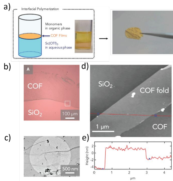
Fig 2. a) Schematic and photograph of liquid-liquid interfacial synthesis process (left) used to prepare TAPB-PDA COF and the resulting free-standing film (right). b) Optical and c) TEM micrographs of TAPB-PDA COF transferred onto Si/SiO 2 substrate and TEM carbon grids, respectively. d) AFM image (white box from b) of isolated monolayer sheets and e) height profile along the red line in d. Adapted with permission from Elsevier. 74
