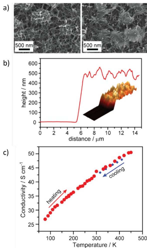
Fig 10. a) SEM micrographs of \text{Ni}_3(\text{HITP})_2 films with 500 nm thickness measured via b) AFM. c) van der Pauw conductivity measurements at various temperatures show reversible increase in conductivity for 500 nm thick films on quartz. Adapted with permission. 168 Copyright 2014 American Chemical Society.
