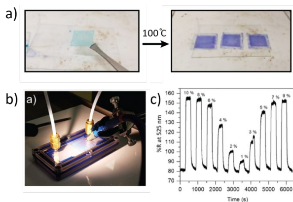
Fig 12. a) Color change from blue to purple upon activation of the HKUST-1 thin films, which were deposited through layer-by-layer methods. b) Photograph of the authors' gas flow cell and reflectance measurement setup. c) Plot of percent reflectance vs. time of HKUST-1 thin films upon their exposure to 0–10% RH for 5 min, followed by 5 min intervals of dry air purge. Adapted with permission. 184 Copyright 2018 American Chemical Society.
