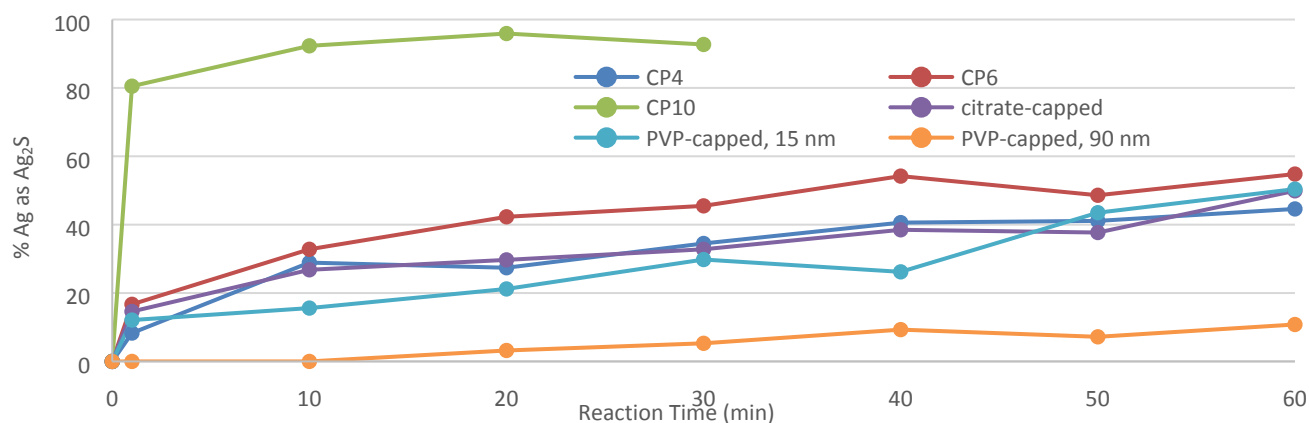
Fig. 1 Silver (I) sulfide formation in the reaction of three AgNP-containing CPs and the three lab-synthesized AgNPs with wastewater sludge.
