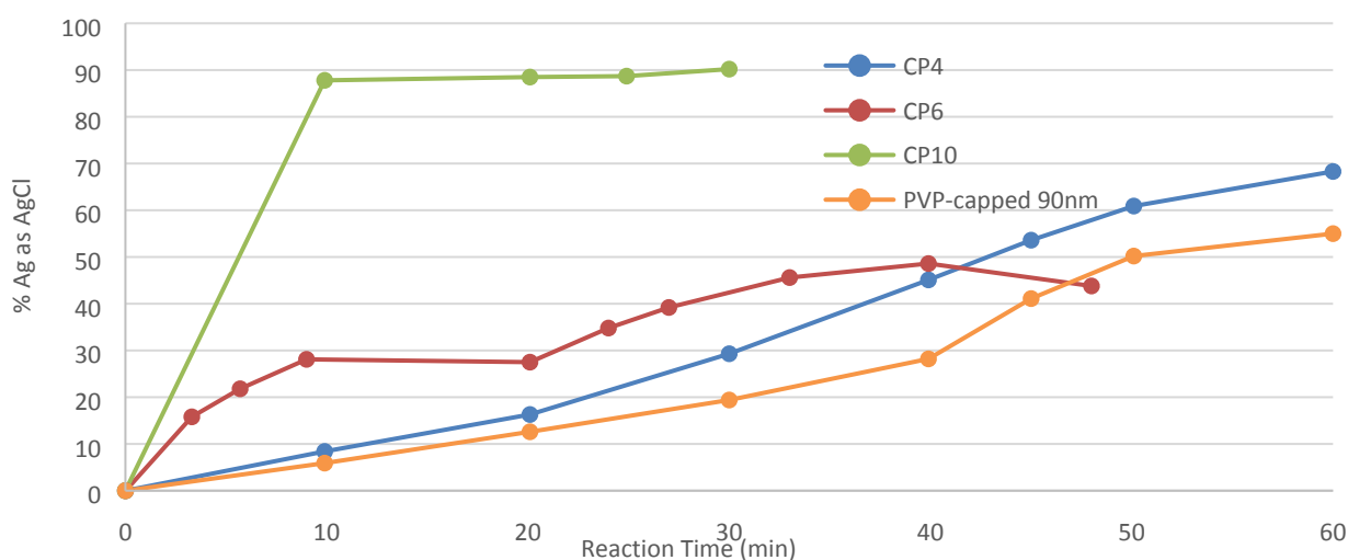
Fig. 2 Silver (I) chloride formation in the reaction of three AgNP CPs and a lab-synthesized AgNP with SSF.
