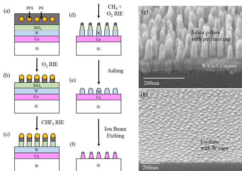
Figure 27. Schematic (a-f) for the fabrication of W-capped Co nanodot arrays using PS- b -PFEMS thin film BCP lithography and TEM images for (g) the preparation of silica pillars
