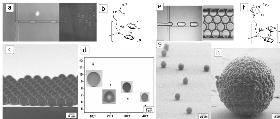
Figure 17. a) Images of head-on forming droplets of PFS (b). c) SEM images of the microgels formed from (b). d) The diameter of PFS (b) microspheres produced at increasing water-to-oil flow rate ratios, e.g. 10: 1 Q_w = 1 \text{ mL min}^{-1} , Q_{\text{PFS}} = 0.1 \text{ mL min}^{-1} . e) Hydrogel precursor droplets of PFS (f) formed in a flow focusing microfluidic device. (g) SEM images of PFS (f) microgels, and (h) SEM image of a single PFS (f) microgel particle. Reproduced with permission from reference 171. Copyright 2014 Royal Society of Chemistry.
