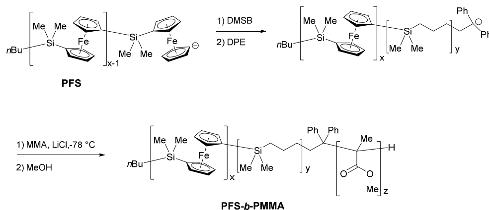
Scheme 13. Synthesis of polyferrocenyldimethylsilane- block -polymethylmethacrylate ( PFMS- b -PMMA ) via reactivity mediation method using DMSB and DPE.
