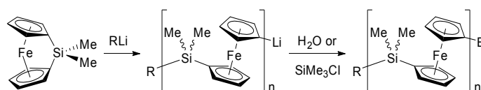
Scheme 5. Living anionic ring opening polymerisation of sila[1]ferrocenophanes. R = \text{Fc} , \text{Ph} , or n -Bu; E = \text{H} or \text{SiMe}_3 .
