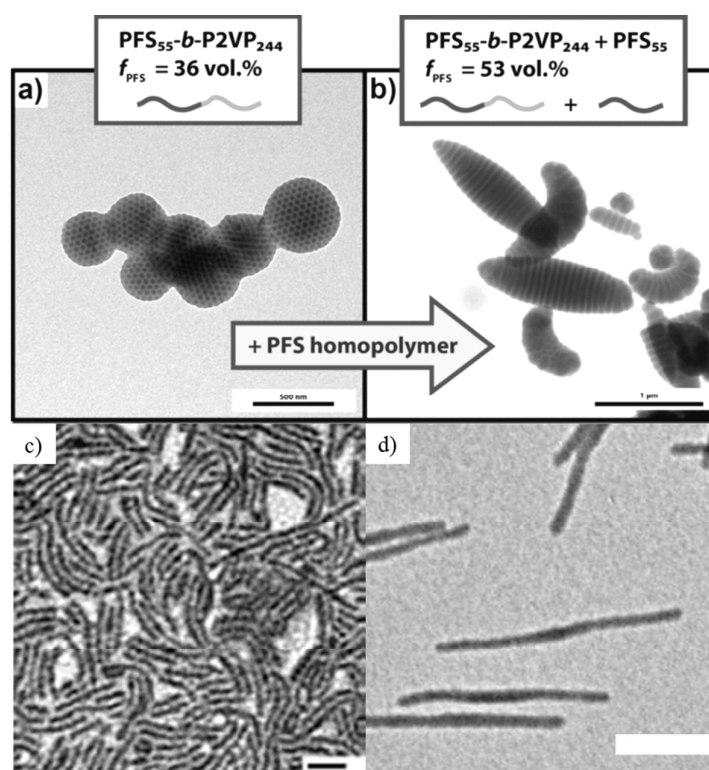
Figure 36. (Top) TEM images showing (a) nanosheets with a hexagonal packed cylinder structure and (b) ellipsoidal particles with an axially stacked lamellar structure formed from blending of PFS - b - P2VP and PFS homopolymer. (Bottom) TEM images showing (c)
