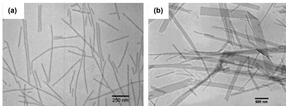
Figure 35. TEM images for the micelles formed from (a) PI 320 - b -PFDMS 53 (6 : 1) and (b) PI 30 - b -PFDMS 60 (1 : 2) in hexane/THF (9:1) and (7:3) respectively. Reproduced with permission from reference 221. Copyright 2002 American Chemical Society.
