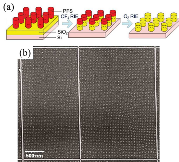
Figure 32. (a) Schematic for formation of pattern transfer to prepare square arrays of silica posts from PI- b -PS- b -PFS diblock copolymer thin films; (b) corresponding SEM image showing highly-ordered square arrays of PFS microdomains within topographical HSQ sidewalls. Reproduced with permission from references 281 280 (copyright 2009 American Chemical Society) and 282 (copyright 2011 American Chemical Society).
