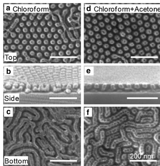
Figure 31. SEM images of PS- b -PFS- b -P2VP diblock copolymer thin films after annealing in (a-c) chloroform and (d-f) a chloroform/acetone mixture for 4 h followed by O 2 RIE; (a, d) plane view, (b, e) side view, (c, f) bottom view. Scale bars are 200 nm. Reproduced with permission from reference 230. Copyright 2009 American Chemical Society.
