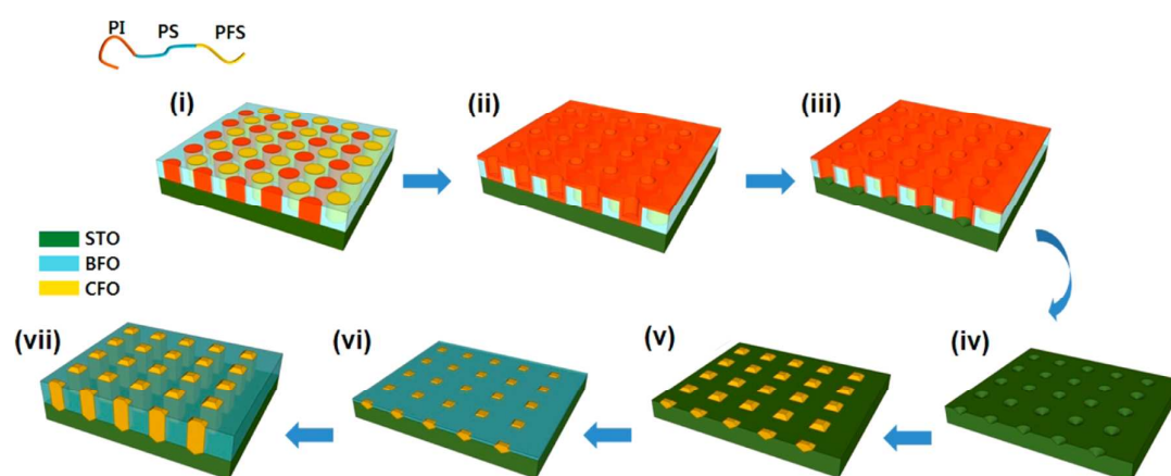
Figure 33. (i-vii) Schematic for the fabrication of a templated BiFeO_3 - CoFe_2O_4 nanocomposite thin film by thin film self-assembly of PI- b -PS- b -PFS/PS blend. Reproduced with permission from reference 314. Copyright 2014 American Chemical Society.
