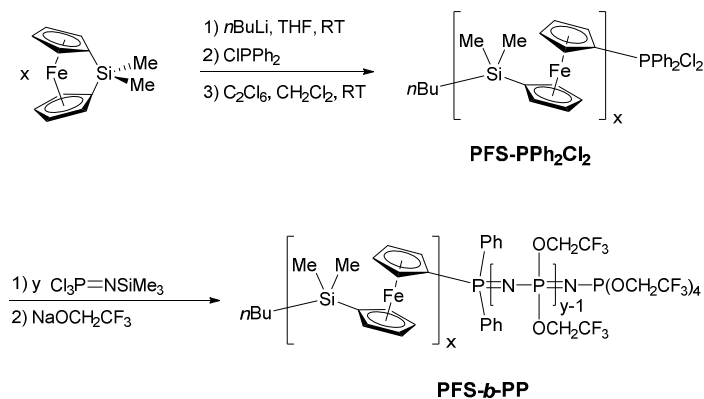
Scheme 16. Synthesis of polyferrocenyldimethylsilane- block -polyphosphazene ( PFDMS- b -PP ).
