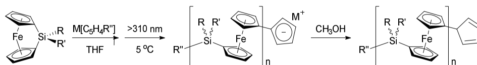
Scheme 6. Photocontrolled living anionic ring opening polymerisation of sila[1]ferrocenophanes.
