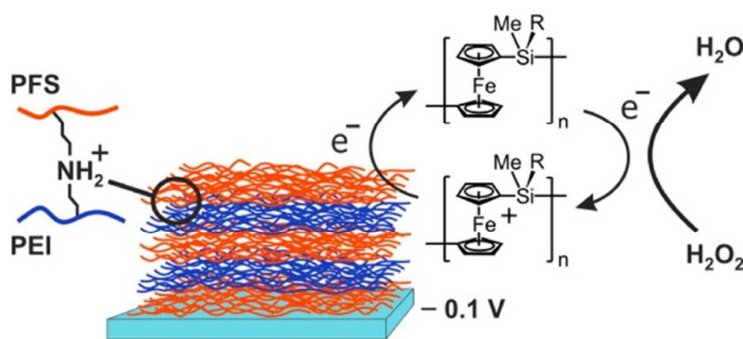
Figure 18. Poly[ferrocenyl(3-bromopropyl)methylsilane] and PEI were employed in a layer-by-layer deposition process to form covalently connected, redox-active multilayer thin films. Upon oxidation and reduction, these covalently interconnected layers do not disassemble, in
