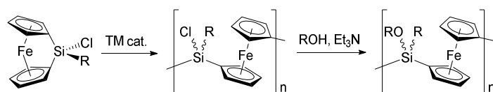
Scheme 4. Transition metal catalysed ROP of a strained sila[1]ferrocenophane, and subsequent main chain functionalisation.
