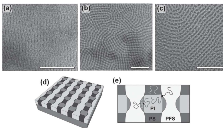
Figure 34. TEM images of \mu -ISF (a) before staining and (b) after staining with \text{OsO}_4 ; (c) SEM image of bottom interface of \mu -ISF; schematics showing (d) thin film pattern and (e) its chain conformation within the microdomain. Scale bars are 300 nm. Reproduced with permission from reference 316. Copyright 2014 American Chemical Society.
