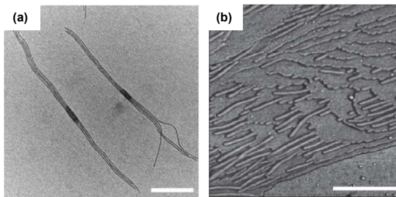
Figure 39. (a) TEM images of “scarf”-like micelles and (b) AFM phase image of cylindrical micelles grown from a PFDMS thin film. Scale bars are 500 nm. Reproduced with permission from reference 357. Copyright 2009 Nature Publishing Group.
