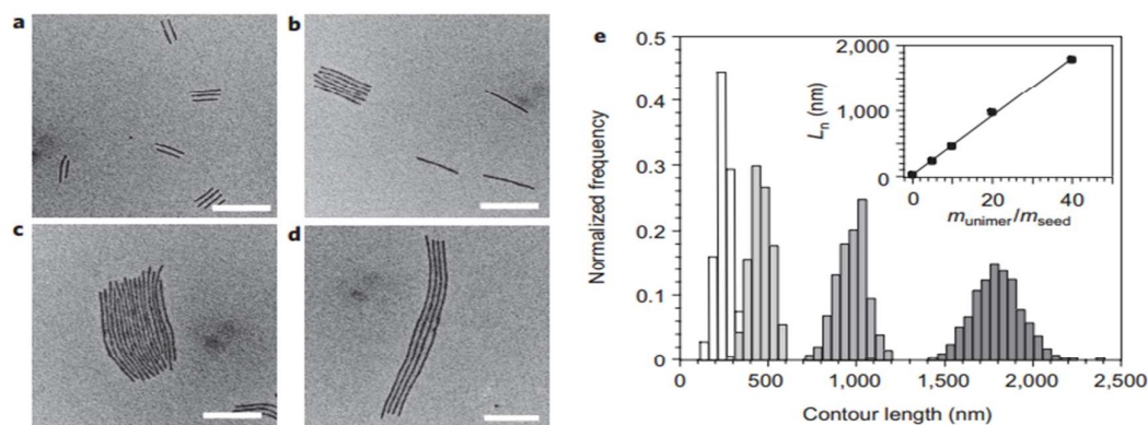
Figure 37. (a-d) TEM images of monodisperse PFDMS- b -PDMS cylindrical micelles grown from uniform stub-like seed micelles with increasing amounts of unimer solution added; (e) histogram of the contour length distribution of the samples; scale bars are 500 nm. Reproduced with permission from reference 325. Copyright 2010 Nature Publishing Group.
