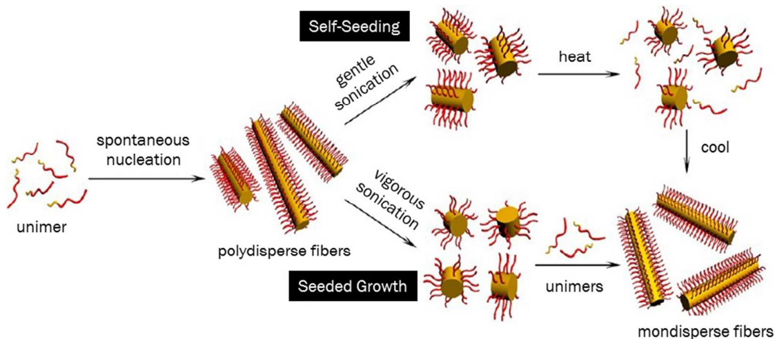
Figure 38. Schematic for the preparation of monodisperse cylindrical micelles by (top) self-seeding and (bottom) seeded growth methods. Reproduced with permission from reference 355. Copyright 2015 American Chemical Society.
