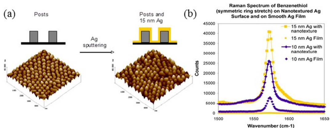
Figure 28. (a) Schematic and corresponding AFM height images for the preparation of a silver nanotextured surface for SERS using a PS- b -PFEMS diblock copolymer thin film; (b) corresponding SERS of benzenethiol on nanotextured Ag films. Reproduced with permission from reference 308. Copyright 2006 Institute of Physics Publishing.
