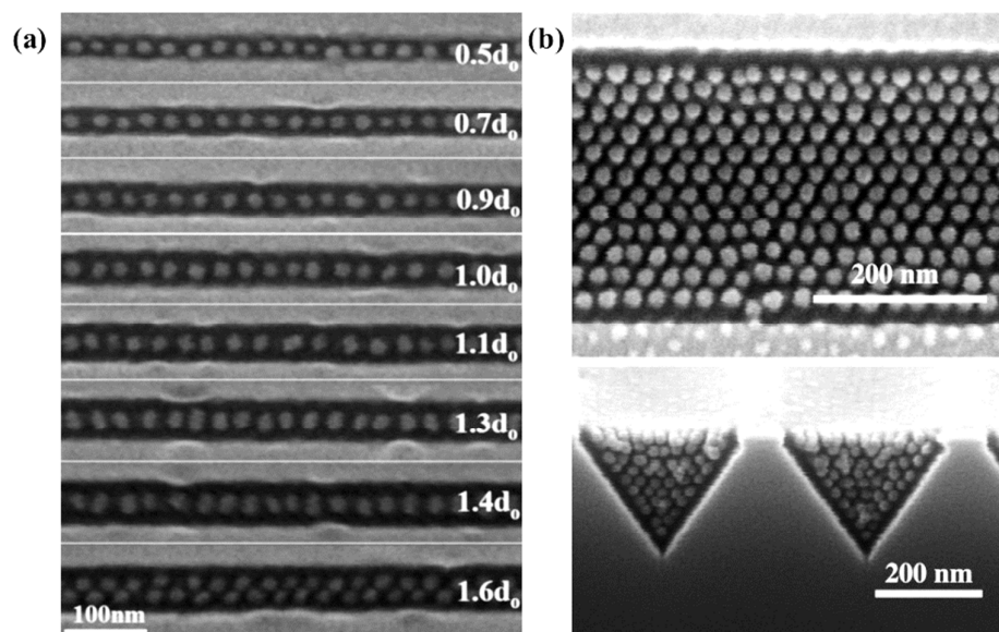
Figure 23. SEM images of PS- b -PFEMS thin films following O_2 RIE in (a) channels of different confinement widths (b) and in V-shaped grooves. Reproduced with permission from references 274 and 275. Copyright 2006 American Chemical Society.
