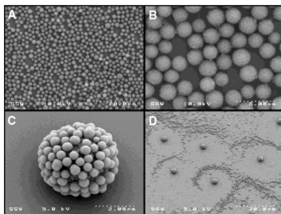
Figure 16. SEM micrographs of: A) PFS microsphere monolayer. B) Higher magnification of a close packed region. C) Negatively charged silica microspheres electrostatically bound to the surface of oxidised polyferrocenylsilane microspheres. D) Surface patterns of core-corona oxidised PFS microsphere-silica assemblies circumscribed by regions of silica spheres. Reproduced with permission from reference 170. Copyright 2001 American Chemical Society.
