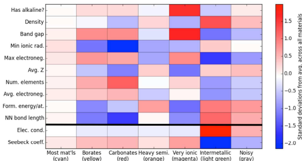
Figure 9: Heat map of selected descriptors used in clustering of materials. The 7 clusters are listed on the x -axis, and the map is used to illustrate the difference in properties between clusters. The thermoelectric properties below the black lines were not used in clustering materials.
