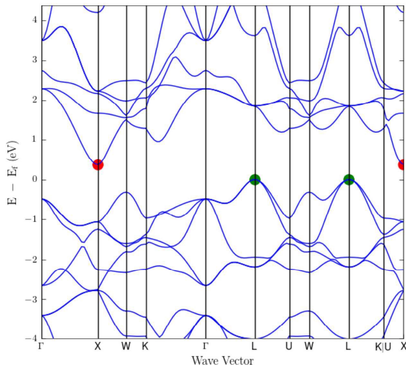
Figure 3: Electronic band structure of NbSbRu (MP materials id = mp-505297) computed using DFT-GGA.
