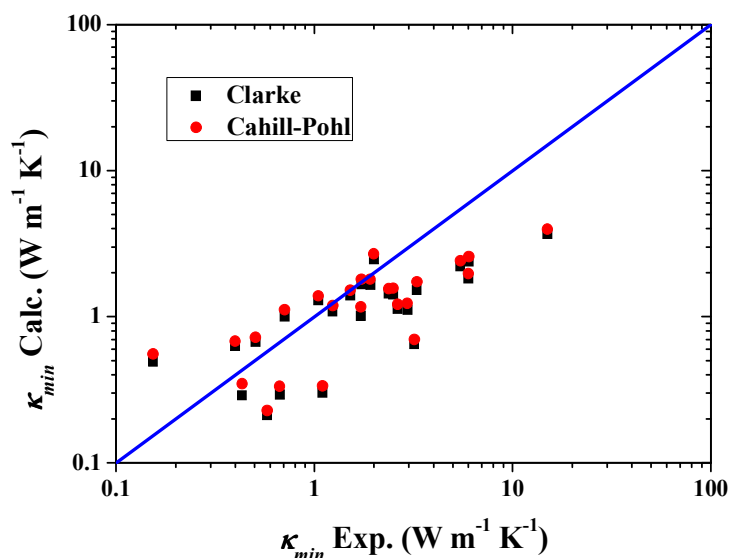
Figure 7: Calculated thermal conductivities in the amorphous limit and experimental minimum thermal conductivities from two models (Clarke and Cahill Pohl) with parameter values computed from DFT-GGA plotted on a log-log scale. The blue line plots equivalence between computation and experiment.
