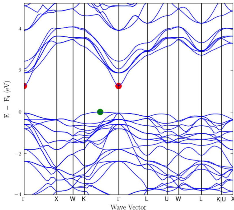
Figure 4: Electronic band structure of \text{Al}_2\text{CdSe}_4 (MP materials id = mp-3807) computed using DFT-GGA.
