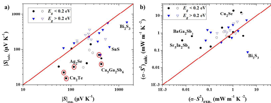
Figure 5: Comparison of the calculated and experimental (a) Seebeck coefficients and (b) power factors for different thermoelectric materials (filled symbols) and the extrinsic doped compounds (hollow symbols). The red circles indicate that the sign of the Seebeck coefficient was incorrect (see Table S1), and the red lines indicate equality of computation and experiment. The calculations are based on the Boltzmann transport equation applied to MP band structures under a constant relaxation time approximation, with temperature and carrier concentration set to conditions where experiments reach the maximum value of the quantity being investigated (Seebeck coefficient in panel (a), power factor in panel (b)). A major source of error appears to be underestimation of band gaps in DFT, as indicated by the poorer agreement for materials with small DFT band gaps (black circles) versus intermediate/large gaps (blue triangles).
