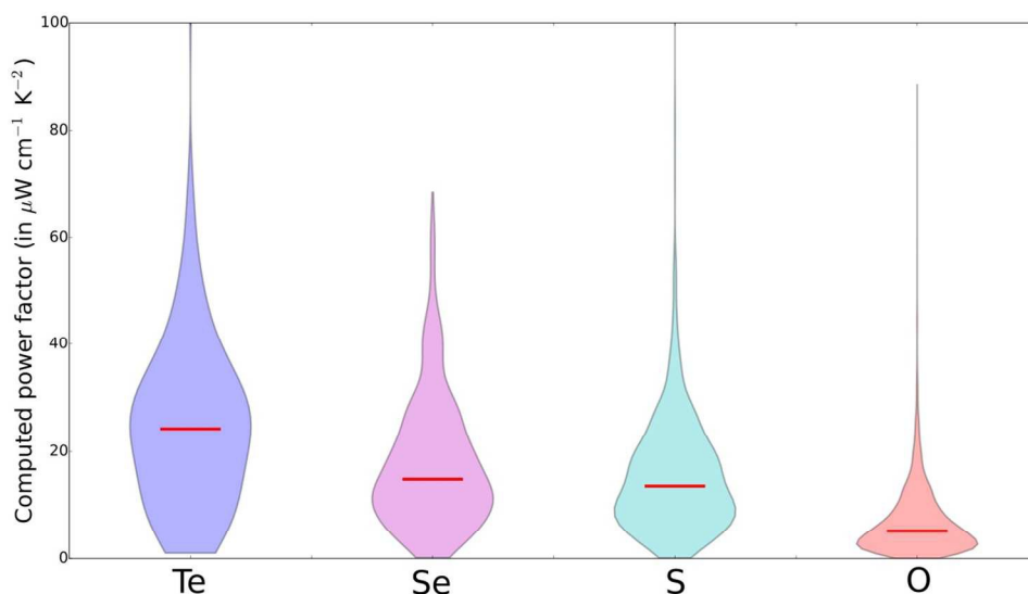
Figure 2: Violin plots depicting the distribution of computed maximum power factor under a fixed relaxation time approximation across compounds in the MP database, separated by anion type. The red lines indicate the median computed power factor for different anions. The distribution of power factors for tellurides tends to be higher than that for selenides and sulfides, which are in turn higher than those of oxides.
