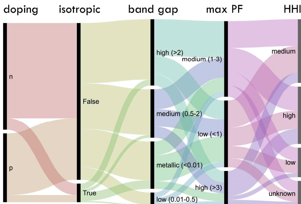
Figure 1: Flow diagram representation of the data set of 48,770 compounds in this study. The term “doping” refers to the doping type that maximizes the power factor in our calculations. Compounds with power factors within 10% in all directions are considered “isotropic”. The unit of band gap is eV and the unit of power factor is \text{mW}\cdot\text{K}^{-2}\cdot\text{m}^{-1} . HHI represents the Herfindahl–Hirschman Index of elemental reserves for the compound and is a measure of the resource criticality of the compound’s component elements, with “high” indicating that resources are geographically confined (undesirable) and “low” indicating geographically dispersed (desirable).
