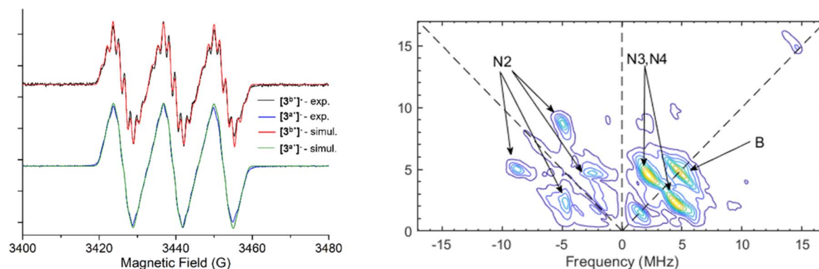
Fig. 4 EPR spectra of [3^{\text{a}}]^{\cdot-} and [3^{\text{b}}]^{\cdot-} , in solution at room temperature, together with their corresponding numerical simulations (left) and HYSCORE spectrum of [3^{\text{b}}]^{\cdot-} recorded at T = 70 K (right).
