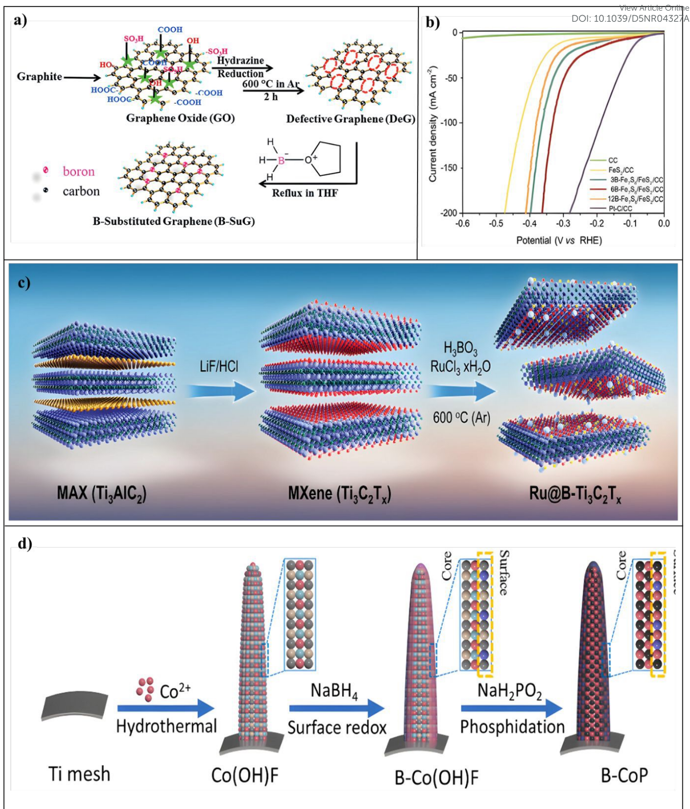
Figure 15. (a) Schematic representation of producing B-substituted graphene (B-SuG). reproduced from Ref. [174] with permission. Copyright 2018, RSC. (b) The B-Fe 7 S 6 /FeS 2 /CC electrocatalysts HER performance in a 1M KOH solution. reproduced from Ref. [45] with permission. Copyright 2022, Wiley. (c) A schematic representation of the synthesis of Ru@B-Ti 3 C 2 T x and Ti 3 C 2 T x . reproduced from Ref. [178] with permission. Copyright 2021, Wiley. (d) Synthesis procedure of B-CoP. reproduced from Ref. [181] with permission. Copyright 2023, Elsevier.
