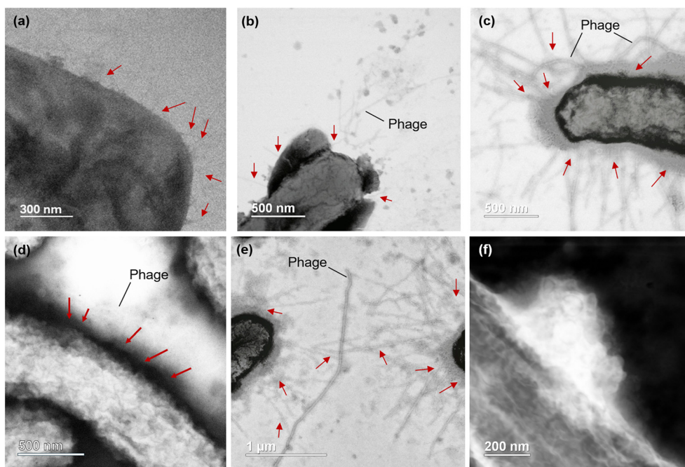
Fig. 6 S/TEM images of E. coli pre-treated with ENMs under light and infected with phage f1: (a) control without ENMs, (b) exposed to 0.2 \text{ mg L}^{-1} n-TiO 2 , (c) exposed to 50 \text{ µg L}^{-1} n-Ag, (d) exposed to 0.2 \text{ mg L}^{-1} n-TiO 2 + 5 \text{ µg L}^{-1} n-Ag mixture, and (e) and (f) exposed to 0.2 \text{ mg L}^{-1} n-TiO 2 + 50 \text{ µg L}^{-1} n-Ag mixture. Fig. 6a–e are in light field TE mode and Fig. 6f is in dark field TE mode, showing the attachment of the ENM mixtures on cell surface (EDS analysis provided in Fig. S10). The red arrows point to the pili/F-pili on bacteria, which are faint and relatively difficult to observe in Fig. 6a, b and d.
