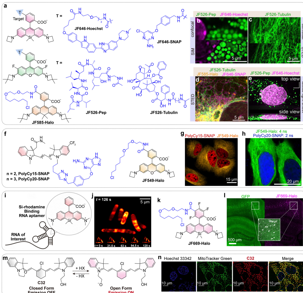
Fig. 24 (a) Chemical structures of various JF labels. (b) Confocal and SIM images of mouse primary hippocampal neurons labeled with JF526 -Pep (green) and JF646 -Hoechst (magenta). (c) Confocal and STED microscopy images of U2OS cells labeled with JF526 -Tubulin (green). (d) Three-color live-cell STED imaging of U2OS cells expressing Sec61 \beta -SNAP-tag labeled with JF646 -SNAP-tag ligand (magenta), TOMM20-HaloTag stained with JF585 -Halo-tag ligand (yellow), and microtubules stained with JF526 -Tubulin (green). (e) Lattice light-sheet microscopy image of U2OS cells stained with JF526 -Pep (green) and JF646 -Hoechst (magenta). Scale bars: 5 \mu m. (f) Chemical structures of the polymethine cyanine label and the JF label used to co-stain cells. (g) Multicolour imaging of live HeLa cells co-transfected with H2B-SNAPf-mTurquoise2 and TUBB5-Halo, and labeled with PolyCy15 -SNAP (red) and JF549 -Halo (orange). Scale bar: 15 \mu m. (h) Fluorescence lifetime multiplexing of the cells co-transfected with H2B-SNAPf-mTurquoise2 and TUBB5-Halo, and incubated with PolyCy20 -SNAP (blue) and JF549 -Halo (green). Scale bar: 20 \mu m. (i) General RNA labeling strategy using a SiR-binding aptamer. (j) STED imaging of live E. coli expressing GFP-SiR mRNA, showing time-lapse images acquired at 31.5 s intervals over 126 s (bottom) and a magnified view at 126 s (top). (k) Chemical structure of JF669 -Halo label. (l) Fluorescent image of a fixed coronal mouse brain slice from an animal expressing GFP-HaloTag fusion protein in neurons after intravenous administration of JF669 -Halo. (m) The pH-modulated spirocyclization equilibrium of C32 . (n) SIM images of HeLa cells co-stained by Hoechst 33342 (blue), MitoTracker Green (green), and C32 (red). Scale bars: 10 \mu m. (b)–(e), (g), (h), (j), (l) and (n) are adapted from ref. 132, 151, 153, 140 and 30 with permission from the American Chemical Society, Springer Nature, the American Chemical Society, Springer Nature and the Chinese Chemical Society, copyright 2019, 2023, 2019, 2020 and 2025, respectively.
