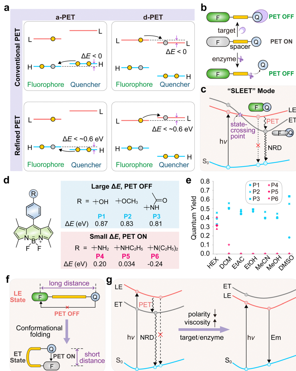
Fig. 7 (a) Schematic representation of the two distinct PET processes (donor-PET named d-PET, and acceptor-PET named a-PET) upon the photoexcitation of a fluorophore. (b) Schematic illustration of PET switch-on and switch-off in probes with a "fluorophore-spacer-receptor" format. F and Q represent the fluorophore and quencher, respectively. (c) Schematic illustration of the state-crossing from a locally excited to an electron-transfer state (SLEET) model. The insets show the conformational changes of probes with a "fluorophore-receptor" format. NRD stands for non-radiative decay. (d) Chemical structures of P1–P6 and their calculated \Delta E values in methanol. (e) Quantum yield values of P1–P6 in various solvents. HEX: n -hexane; DCM: dichloromethane; EtAc: ethyl acetate; EtOH: ethanol; MeCN: acetonitrile; MeOH: methanol; DMSO: dimethyl sulfoxide. (f) Conformational changes that activate the PET process in probes with a "fluorophore-spacer-receptor" format, highlighting the dynamic nature of this process. (g) Schematic illustration of the switch-on and switch-off of PET probes in response to microenvironmental changes or interactions with target molecules or enzymes.
