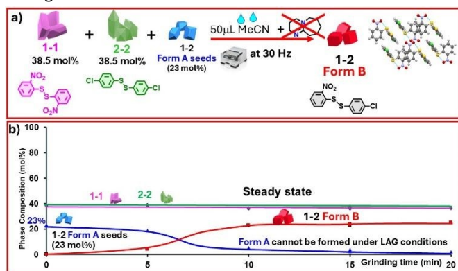
Figure 26 LAG reaction of 1-1 and 2-2 with seeds of 23 mol% short-lived crystals of Form A in the absence of DBU. (a) Reaction scheme (b) Kinetic profile prepared from Rietveld refinements data of PXRD scans. Each point in the kinetic profile represents an independent experiment. 51 Adapted from Ref 51 with permission from JACS, 2014, 136, 16156-16166, Copyright {2014} American Chemical Society.
