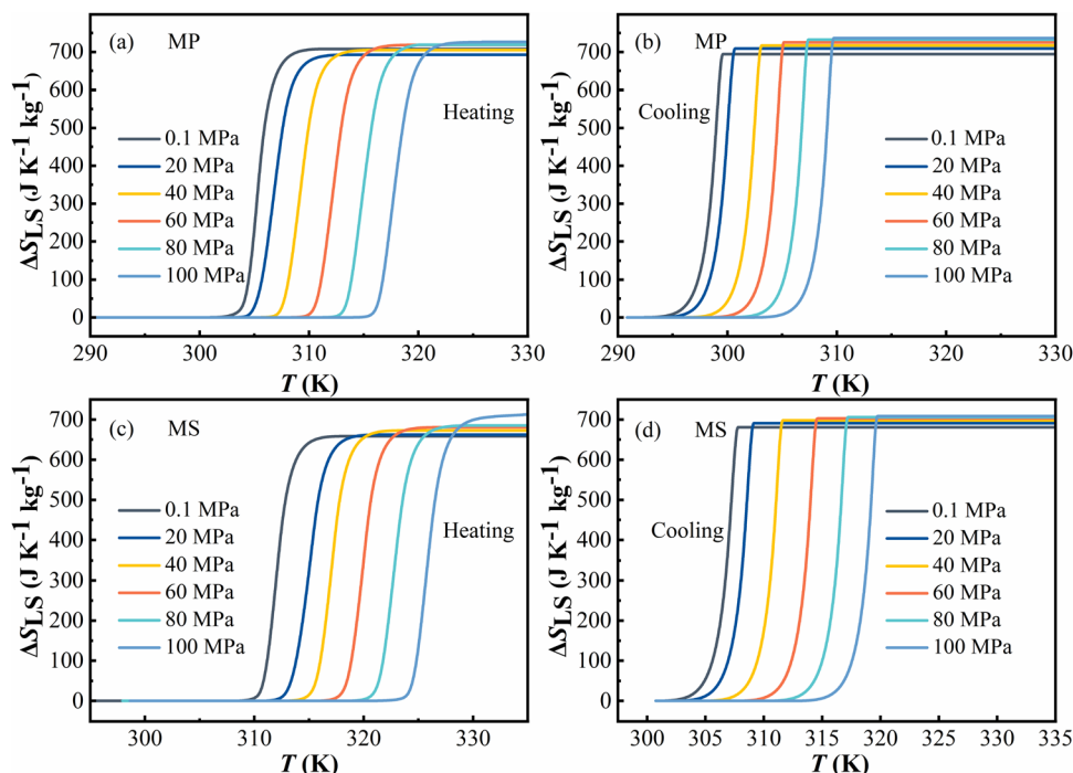
Fig. 3 Entropy changes \Delta S_{LS} in L-S-T during heating and cooling processes at P = 0.1, 20, 40, 60, 80 and 100 MPa. (a) and (b) Methyl palmitate (MP) and (c) and (d) methyl stearate (MS).
