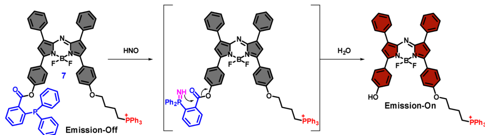
Fig. 7 Turn on mechanism of NIR mitochondrial probe 7 for HNO detection. (Redrawn the ChemDraw structures from ref. 77).
