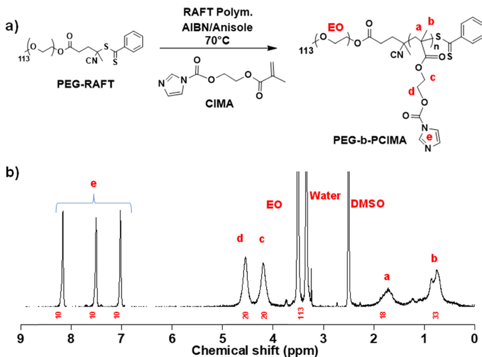
Fig. 2 Synthesis via RAFT polymerization (a) and ^1\text{H} NMR spectrum in \text{DMSO}-d_6 of the \text{PEG-}b\text{-PCIMA} block copolymer. Conditions: [\text{CIMA}]_0/[\text{PEG-RAFT}]_0/[\text{AIBN}]_0 = 100/1/0.5 ; CIMA/anisole (w/w) = 1/0.6.
