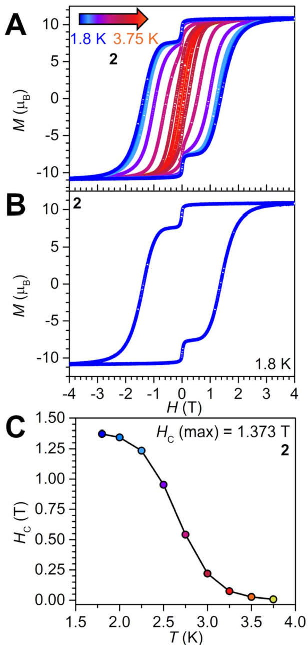
Fig. 10 Plot of magnetisation ( M ) vs. dc magnetic field ( H ) at an average sweep rate of 0.01 \text{ T s}^{-1} for 2 : (A) from 1.8 to 3.75 K, and (B) at 1.8 K. (C) Plot of coercive field vs. temperature for 2 , where solid line is a guide for the eye.
