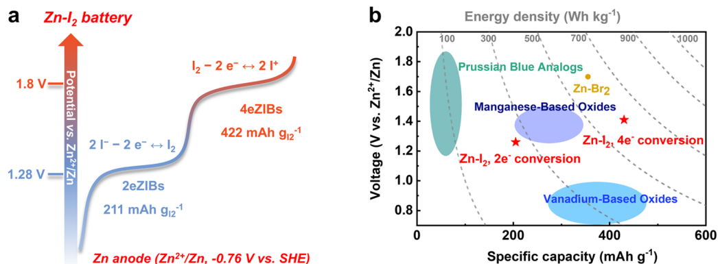
Fig. 1 Comparison of energy density of ZIBs with existing AZBs. (a) Schematic for iodine conversion. (b) Theoretical energy density of commonly used cathodes for AZBs.
