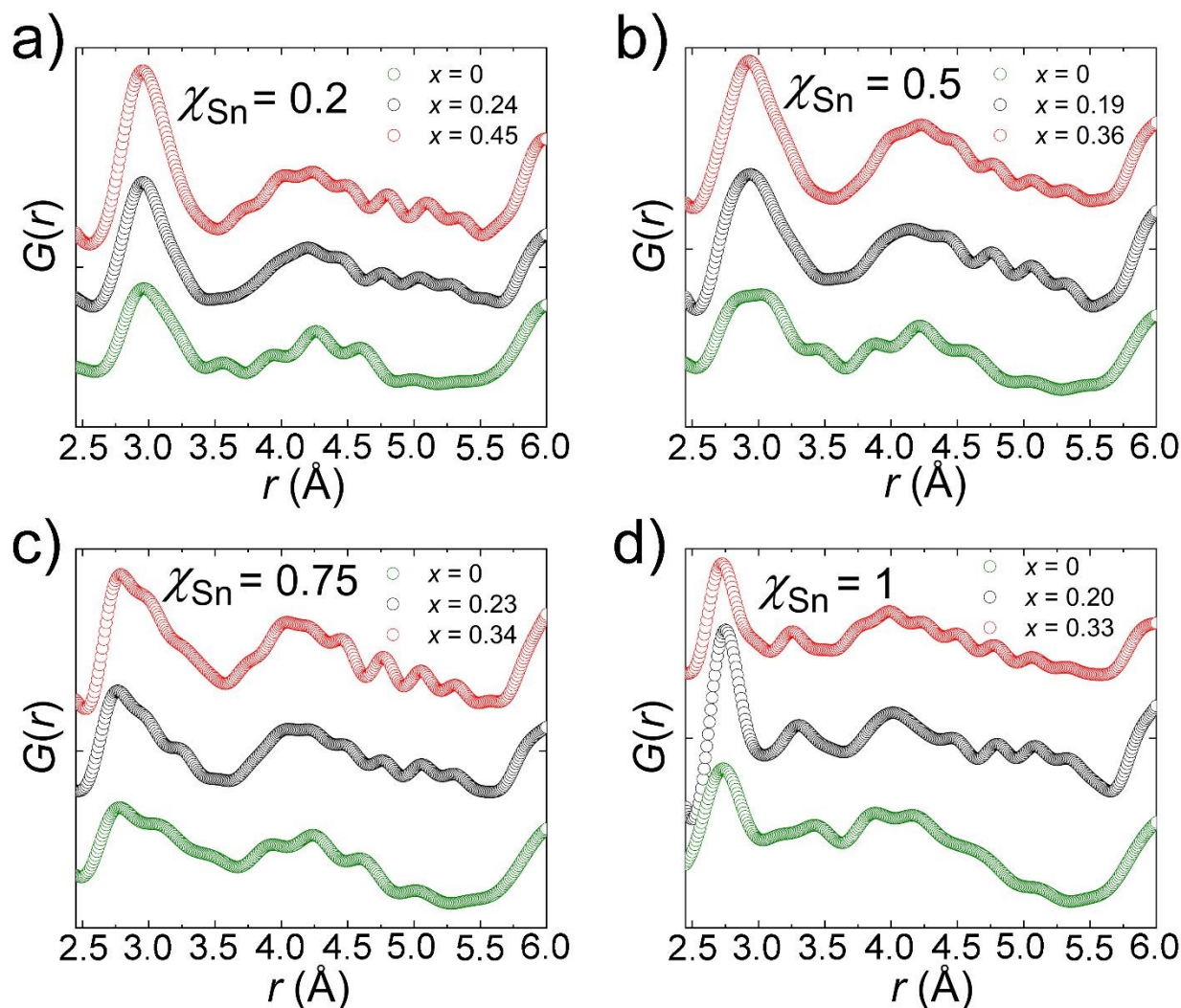
Figure 7: Experimental pair distribution function (PDF) curves for representative compounds in the \text{FA}_{1-x}\text{en}_x\text{Pb}_{\eta-y}\text{Sn}_{\gamma}\text{Br}_3 family of perovskites in four panels (a, b, c, & d) depending on the experimentally determined Sn fraction ( \chi_{\text{Sn}} ) and ethylenediammonium fraction ( x ). Here the PDF of \text{FASnBr}_3 is plotted from our previous works for comparison. 51
