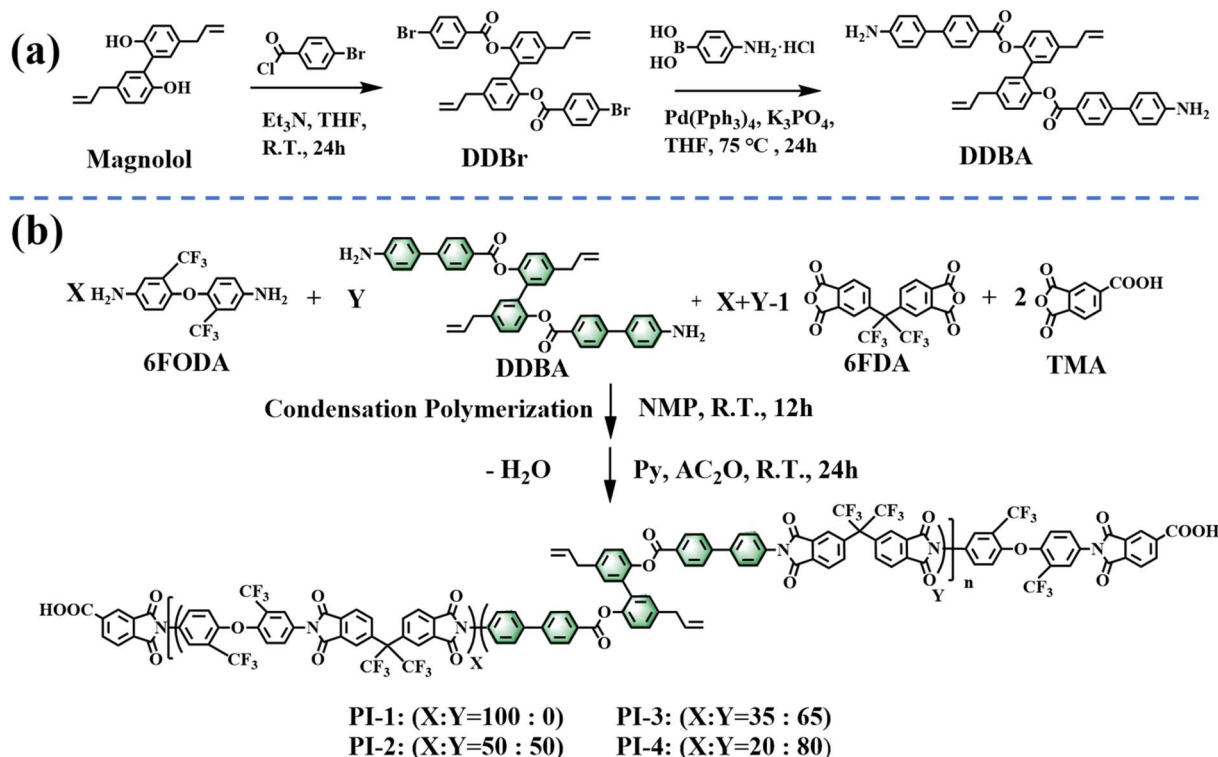
Fig. 2 Synthetic routes of (a) DDBA and its intermediate products and (b) polyimides.
