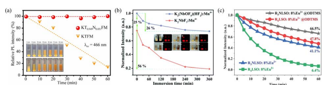
Fig. 6 (a) Relative emission intensity ( \lambda_{\text{ex}} = 466 nm) and photographs of K 2 Ti 0.949 Nb 0.051 F 6.051 :5.0%Mn 4+ (the upper illustration) and K 2 TiF 6 :5.0%Mn 4+ (the inferior illustration) after immersion in deionized water for different times. Reproduced with permission from ref. 153. Copyright 2021, Elsevier. (b) Normalized emission intensity and photographs of K 3 (NbOF 5 )(HF 2 ):Mn 4+ and K 2 NbF 7 :Mn 4+ red phosphors at 630 nm after various immersion times. Reproduced with permission from ref. 155. Copyright 2019, the Royal Society of Chemistry. (c) Time-dependent normalized PL intensities of R 3 NLSO:8%Eu 2+ @ODTMS, R 4 LSO:8%Eu 2+ @ODTMS, R 3 NLSO:8%Eu 2+ , and R 4 LSO:8%Eu 2+ immersed in water. Reproduced with permission from ref. 157. Copyright 2021, WILEY-VCH.
