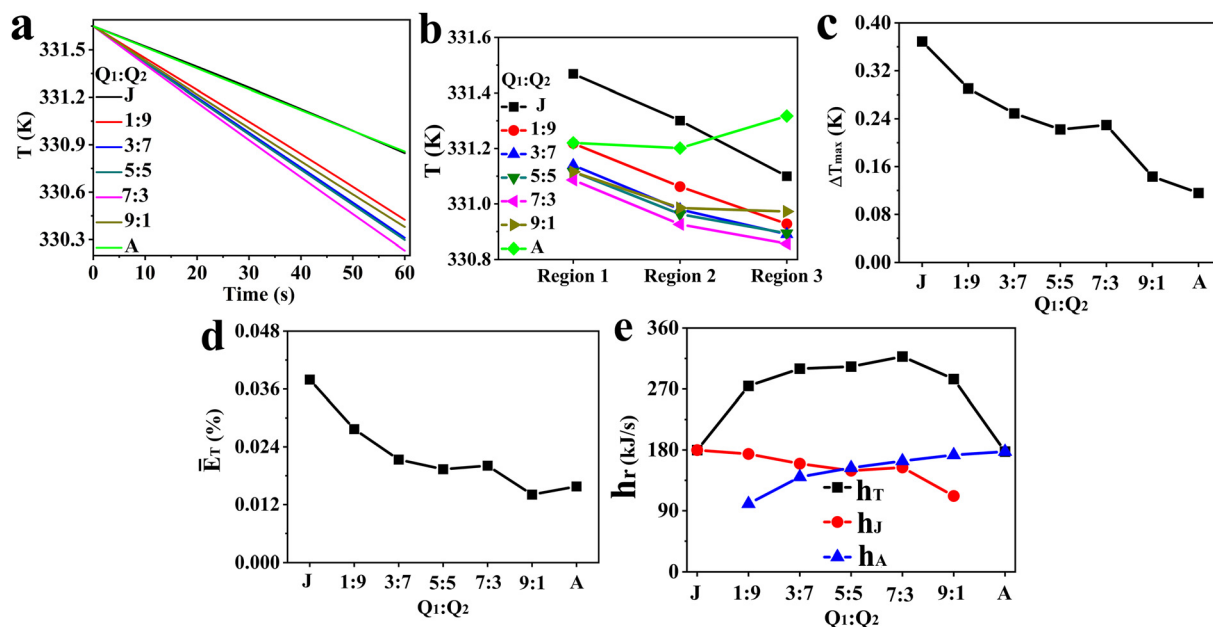
Fig. 4 Effect of Q_1:Q_2 on (a) fluid temperature in the reaction zone at different times, (b) average fluid temperature in various regions, (c) \Delta T_{max} , (d) E_T , and (e) h_T , h_A , h_J (J and A correspond to all cooling water entering the jacket and the agitator, respectively).
