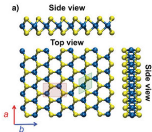
Fig. 3 Atomic structure of two-dimensional transition-metal dichalcogenides (TMDs) of the general formula \text{MX}_2 , where \text{M} = \text{Mo}, \text{W} , or \text{Ti} . The schematic highlights the layered arrangement, in which a transition-metal atom sheet is sandwiched between two chalcogen atom layers, as well as the in-plane lattice vectors ( a and b ). This unique architecture imparts TMDs with tunable band gaps, high surface area, and strong light–matter interactions, making them promising candidates for applications such as antioxidant stabilization, photothermal antimicrobial packaging, and stimuli-responsive nutraceutical delivery. The figure is obtained from ref. 42 under a Creative Common (CC BY) License.
