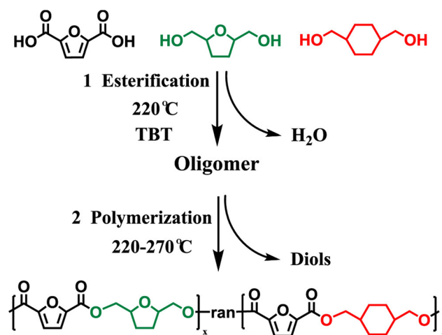
Fig. 3 Schematic representation of the synthesis of poly(1,4-cyclohexyldimethylene-co-hydroxymethyl tetrahydrofuran 2,5-furandicarboxylate) (PCTF) from FDCA, BHMTHF and CHDM. Figure adapted and reproduced with permission from ref. 37. Copyright 2021 ACS Sustainable Chem. Eng.
