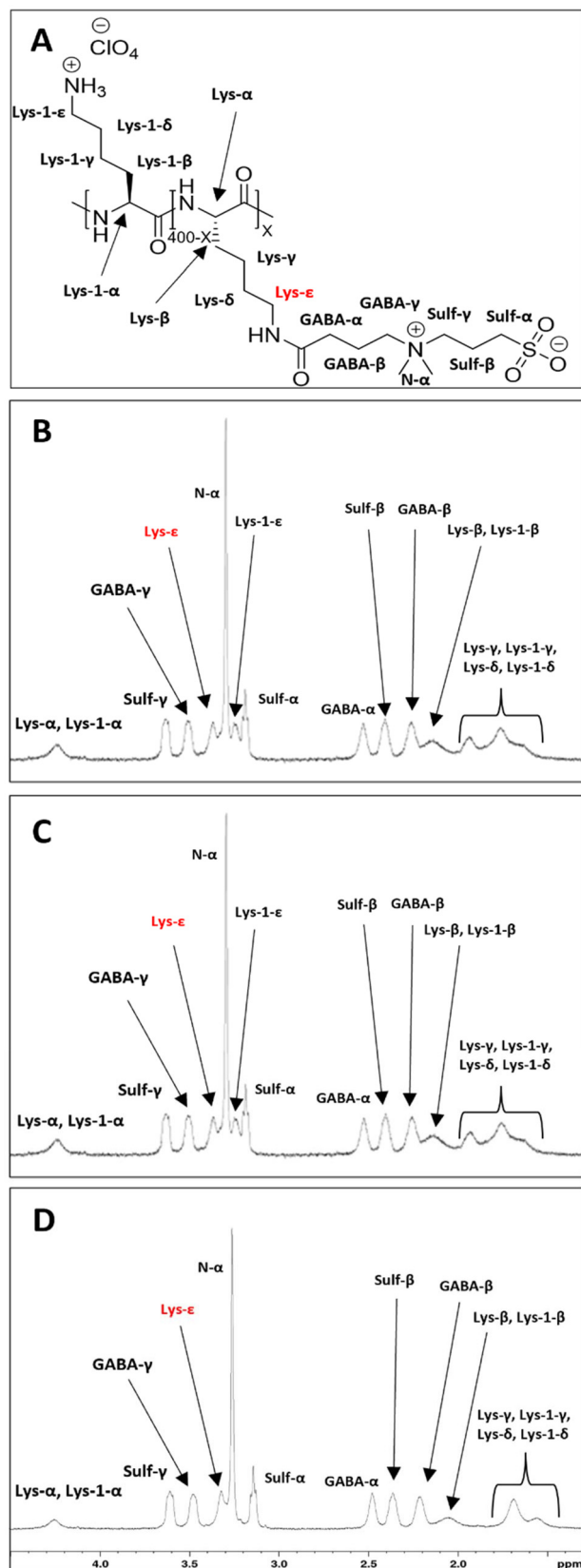
Fig. 3 ^1\text{H} NMR spectra (500 MHz, \text{D}_2\text{O} ) of \alpha -PLL functionalized with zwitterion 9. (A) Structures of polymers 12a–12e , X = 44–396 . (B) 31%, (C) 63%, and (D) 99% functionalization.
