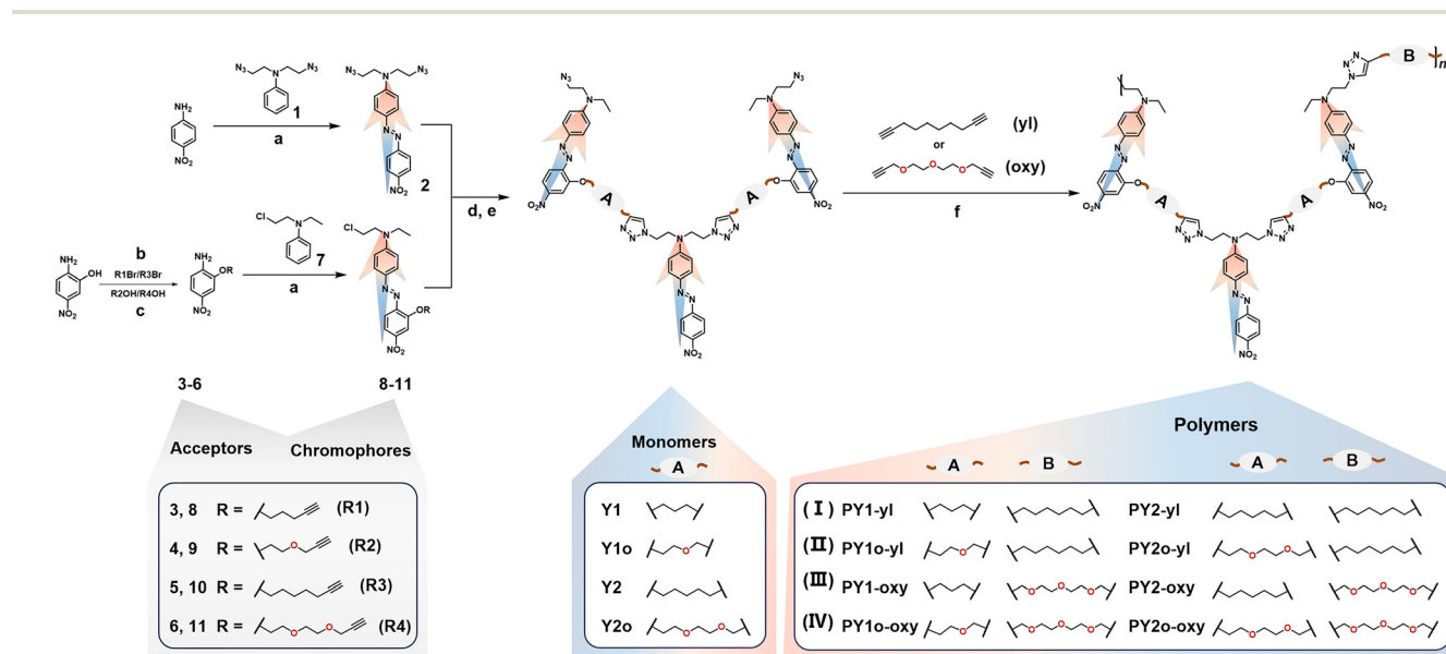
Scheme 1 The synthetic routes of target polymers and the corresponding structure characterization. Reaction conditions: (a) HCl (38%), \text{NaNO}_2/\text{H}_2\text{O} , \text{CH}_3\text{CN} , 0–5 °C; (b) \text{K}_2\text{CO}_3 , DMF, 80 °C; (c) DIAD \text{PPh}_3 , THF, 30 °C; (d) \text{CuSO}_4 \cdot \text{H}_2\text{O} , VcNa, THF/ \text{H}_2\text{O} , 30 °C; (e) \text{NaN}_3 , DMF, 80 °C; (f) \text{CuSO}_4 \cdot \text{H}_2\text{O} , VcNa, DMF, 25 °C.
