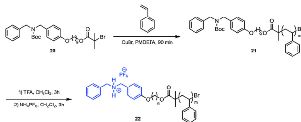
Scheme 5 Synthesis of telechelic PS-DBA + , 22.
