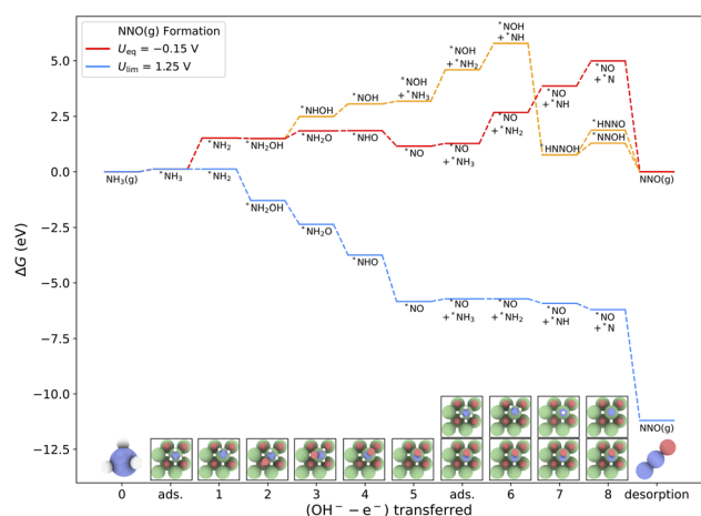
Fig. 15 Free energy diagram for N_2O(g) formation by proceeding through the interaction between *NO and *N (Langmuir–Hinshelwood recombination). After *NH_2OH is formed, the mechanism branches towards *NHOH or *NH_2O , with the latter deprotonation step being energetically preferred. This pathway requires the subsequent deprotonation steps to form *N . Equilibrium (red trace) and limiting (blue trace) potentials are calculated using the computational hydrogen electrode at pH 11. The coupling between *NOH and *NH to avoid the thermodynamically unfavourable chemical step of the proton transfer is shown as well (orange trace).
