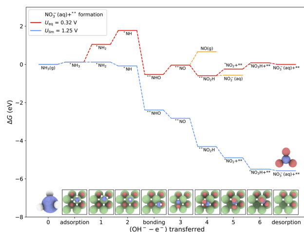
Fig. 16 Free energy diagram for NO(g) , NO_2^-(aq) , and NO_3^-(aq) formation by proceeding through the interaction between *N -containing intermediates and the lattice oxygen, **O_{lat} . The energies of desorption for NO(g) , NO_2^-(aq) , and NO_3^-(aq) were calculated to be +0.77, +0.19, and -0.74 eV, respectively. Equilibrium (red trace) and limiting (blue trace) potentials were calculated using the computational hydrogen electrode at pH 11.
