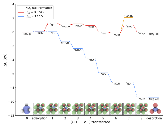
Fig. 14 Free energy diagram for \text{NO}_3^- (aq) formation by proceeding through the same mechanistic steps towards \text{NO}_2^- (aq). After *\text{NO}_2\text{H} is formed, the mechanism branches towards *\text{NO}_2 or *\text{NO}_3\text{H}_2 , with the deprotonation step being energetically preferred. The energy required for the final desorption step was calculated to be -0.029 eV. Equilibrium (red trace) and limiting (blue trace) potentials are calculated using the computational hydrogen electrode at pH 11.
